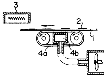
FIG. 2 (PRIOR ART)
