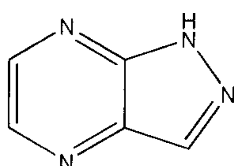
1H-pyrazolo[4,3-b]pyrazine
