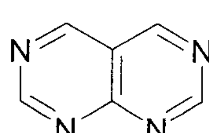
pyrimido[4,5-d]pyrimidine (pyrimido[4,5-d]pyrimidinyl)
