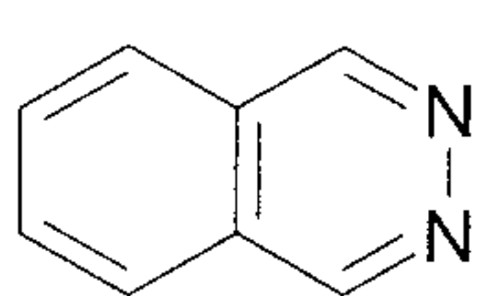
phthalazine (phthalazinyl)
