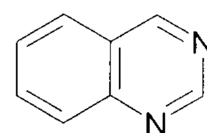
quinazoline (azaquinazoline)
