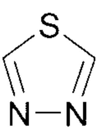
1-thia-3,4-diazole (1-thia-3,4-diazolyl)
