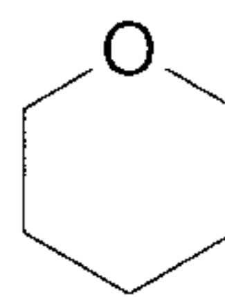
tetrahydropyran (tetrahydropyranyl)
