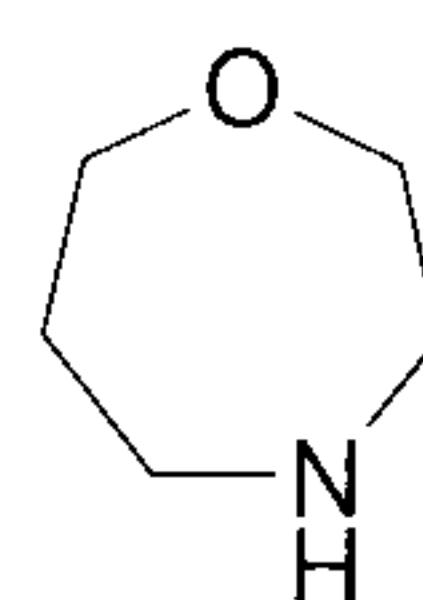
1,4-oxaazepane (1,4-oxaazepanyl)
