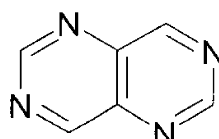
pyrimido[5,4-d]pyrimidine (pyrimido[5,4-d]pyrimidinyl)
