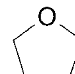
tetrahydrofuran (tetrahydrofuranyl)
