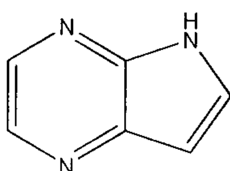
5H-pyrrolo[3,2-b]pyrazine
