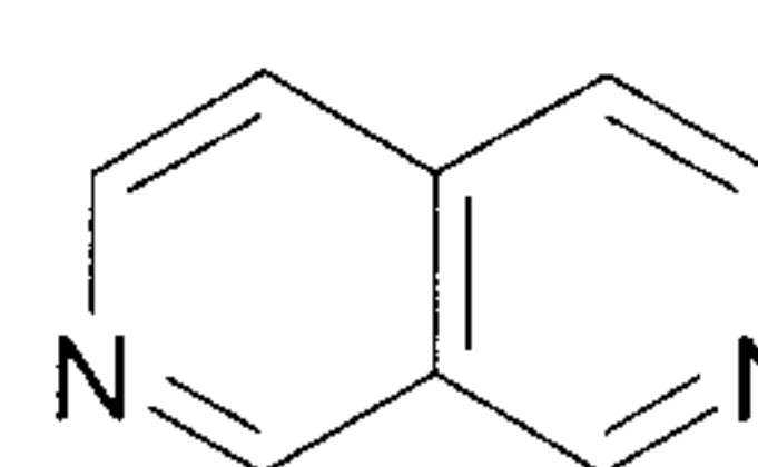
2,7-naphthyridine (2,7-naphthyridinyl)
