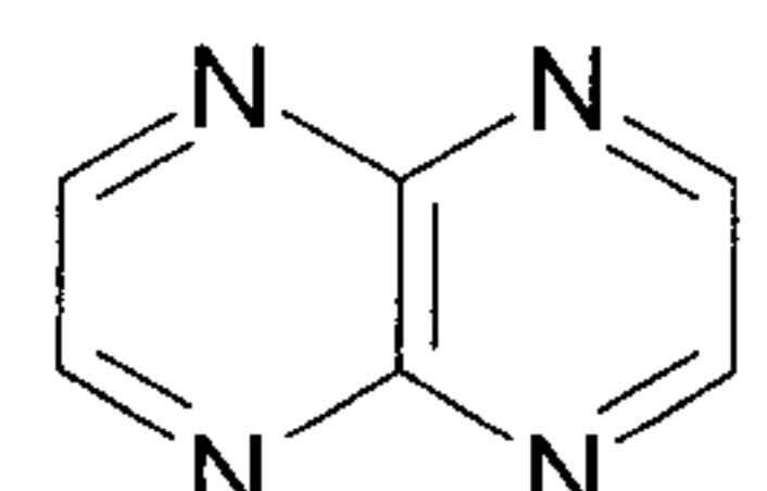
pyrazino[2,3-b]pyrazine (pyrazino[2,3-b]pyrazinyl)
