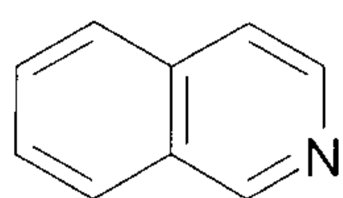
isoquinoline (isoquinolinyl)
