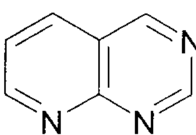
pyrido[2,3-d]pyrimidine (pyrido[2,3-d]pyrimidinyl)
