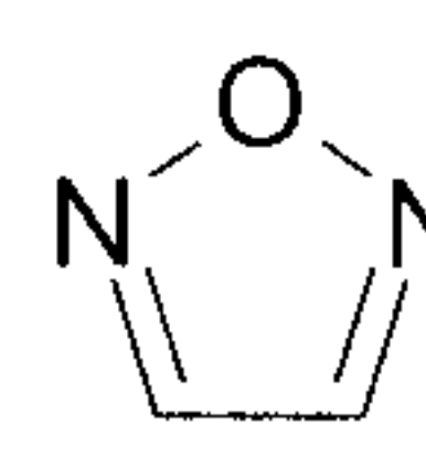
1-oxa-2,5-diazole (1-oxa-2,5-diazolyl)
