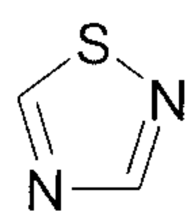
1-thia-2,4-diazole (1-thia-2,4-diazolyl)
