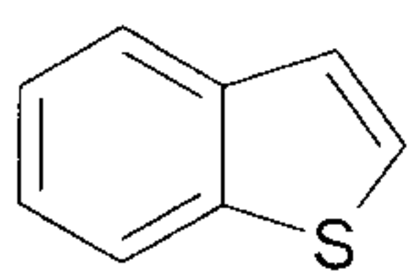
benzothiophene (benzothiophenyl)
