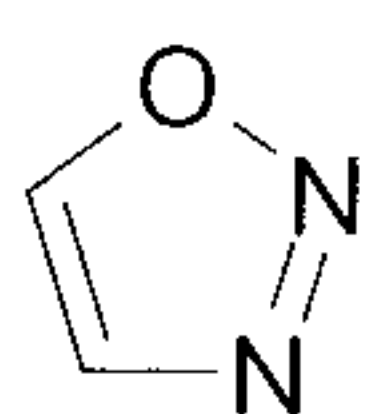
1-oxa-2,3-diazole (1-oxa-2,3-diazolyl)
