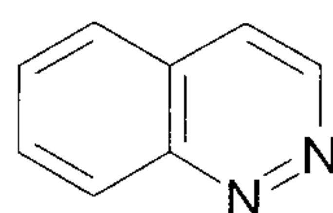
cinnoline (cinnolinyl)
