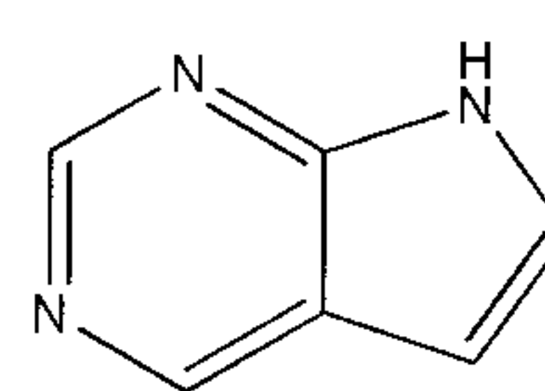
7H-pyrrolo[2,3-d]pyrimidine
