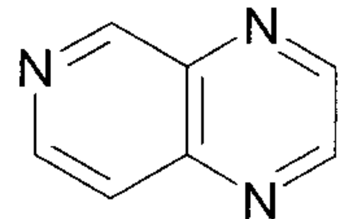
pyrido[3,4-b]pyrazine (pyrido[3,4-b]pyrazinyl)
