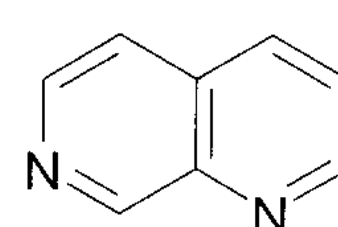
1,7-naphthyridine (1,7-naphthyridinyl)
