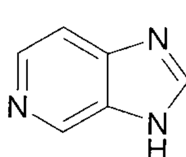
imidazo[4,5-c]pyridine (imidazo[4,5-c]pyridinyl)
