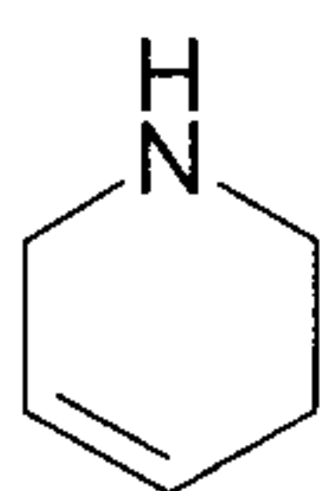
1,2,5,6-tetrahydropyridine (1,2,5,6-tetrahydropyridinyl)
