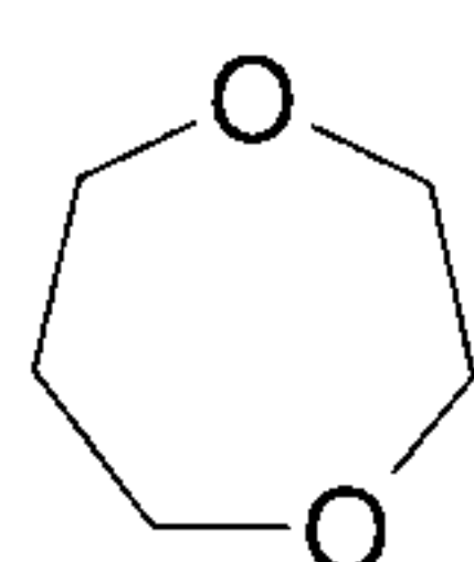
1,4-dioxepane (1,4-dioxepanyl)
