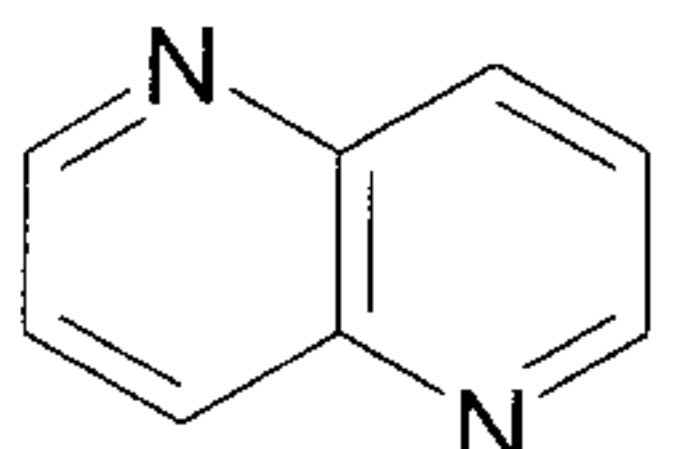
1,5-naphthyridine (1,5-naphthyridinyl)
