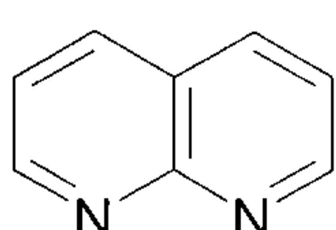
1,8-naphthyridine (1,8-naphthyridinyl)
