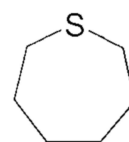
thiepane (thiepanyl)
