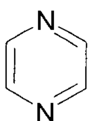
pyrazine (pyrazinyl)
