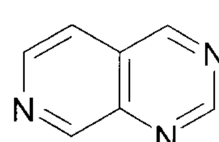
pyrido[3,4-d]pyrimidine (pyrido[3,4-d]pyrimidinyl)
