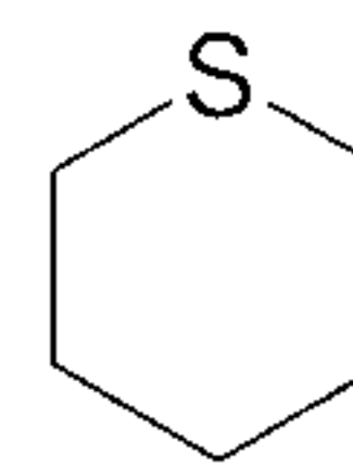
tetrahydrothiopyran (tetrahydrothiopyranyl)
