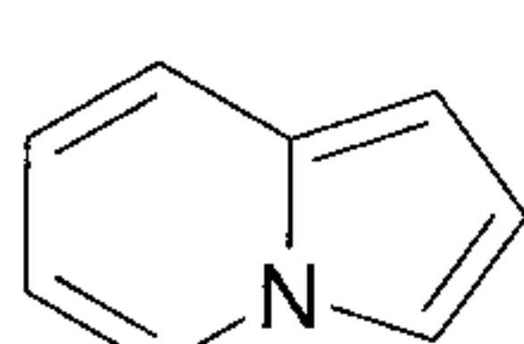
indolizine (indolinyl)
