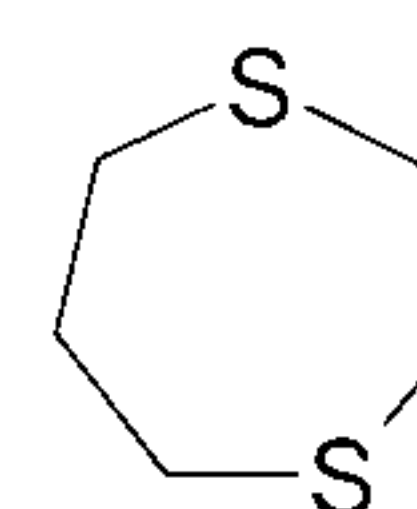
1,4-dithiepane (1,4-dithiepanyl)
