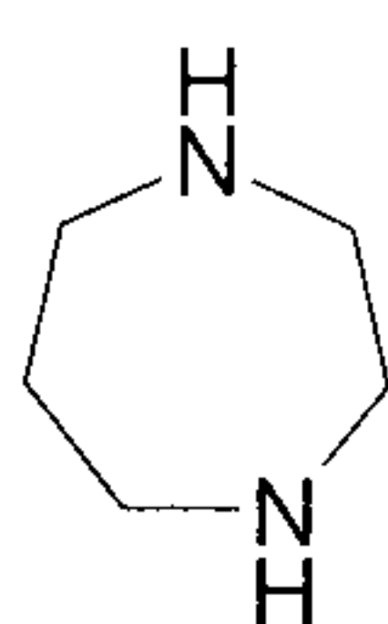
1,4-diazepane (1,4-diazepanyl)
