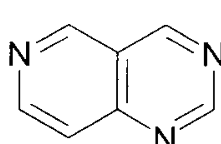
pyrido[4,3-d]pyrimidine (pyrido[4,3-d]pyrimidinyl)
