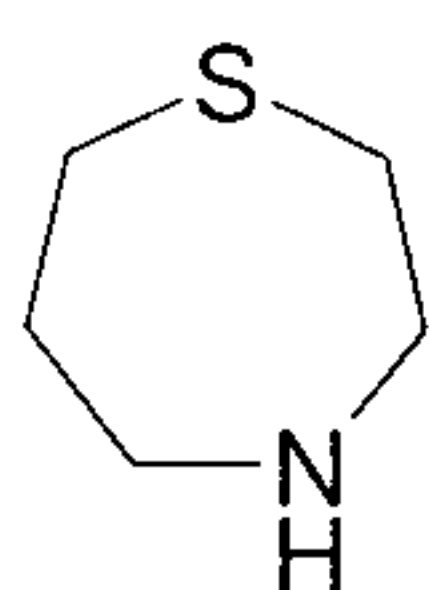
1,4-thieazepane (1,4-thieazepanyl)
