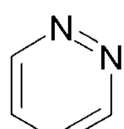
pyridazine (pyridazinyl)
