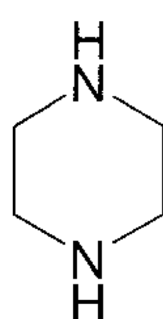
piperazine (piperaziny)
