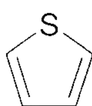
thiophene (thiophenyl)
