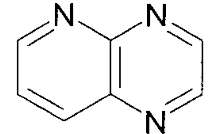
pyrido[2,3-b]pyrazine (pyrido[2,3-b]pyrazinyl)
