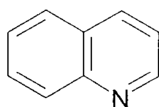
quinoline (quinolinyl)
