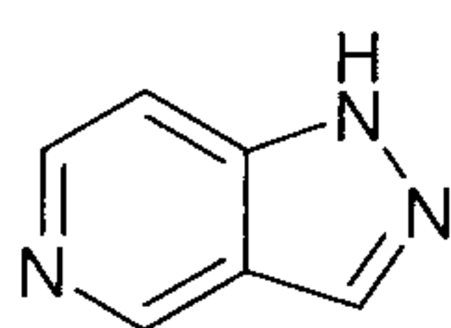
pyrazolo[4,3-c]pyridine (pyrazolo[4,3-c]pyridinyl)
