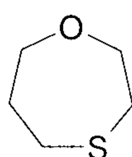
1,4-oxathiepane (1,4-oxathiepanyl)
