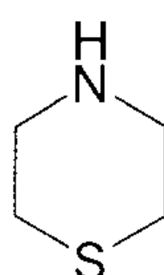
1,4-azathiane (1,4-azathianyl)
