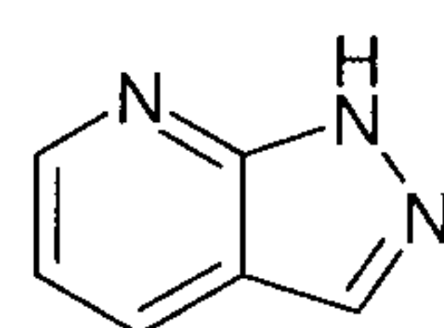
pyrazolo[3,4-b]pyridine (pyrazolo[3,4-b]pyridinyl)
