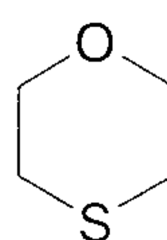
1,4-oxathiane (1,4-oxathianyl)
