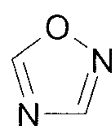
1-oxa-2,4-diazole (1-oxa-2,4-diazolyl)
