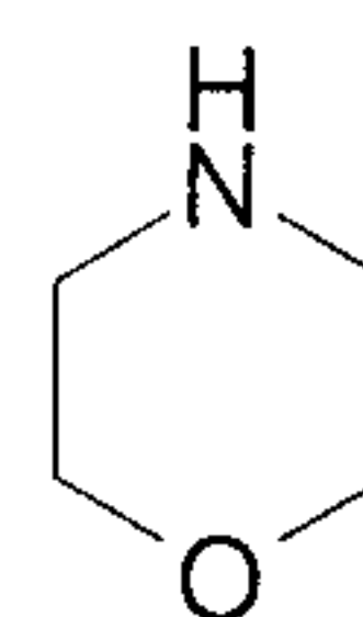
morpholine (morpholiny)
