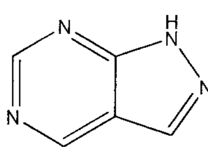
1H-pyrazolo[3,4-d]pyrimidine
