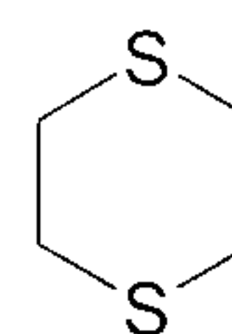
1,4-dithiane (1,4-dithianyl)
