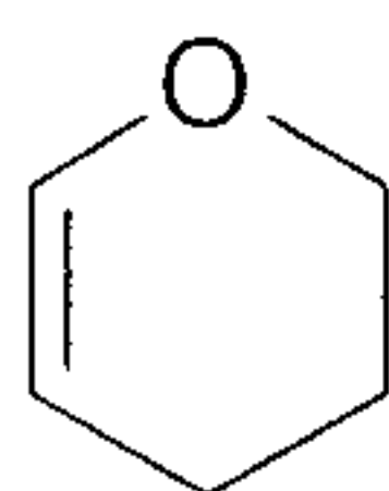
3,4-dihydro-2H-pyran (3,4-dihydro-2H-pyranyl)
