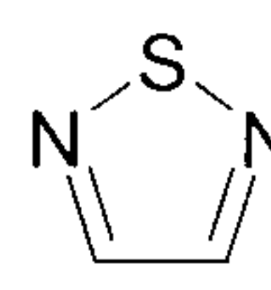
1-thia-2,5-diazole (1-thia-2,5-diazolyl)
