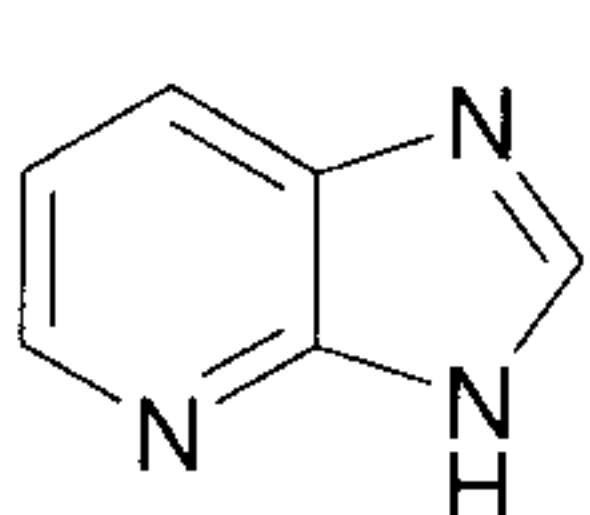
imidazo[4,5-b]pyridine (imidazo[4,5-b]pyridinyl)
