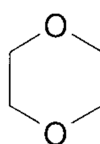
1,4-dioxane (1,4-dioxanyl)
