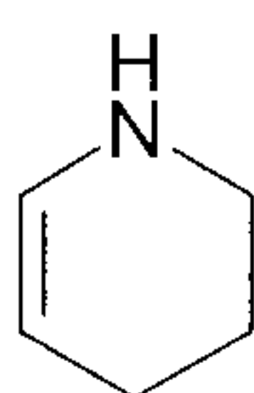
1,2,3,4-tetrahydropyridine (1,2,3,4-tetrahydropyridinyl)
