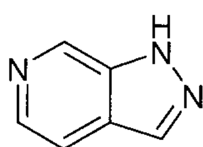
pyrazolo[3,4-c]pyridine (pyrazolo[3,4-c]pyridinyl)
