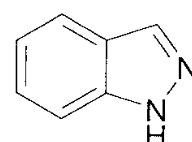
indazole (indazolyl)
