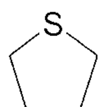
tetrahydrothiophene (tetrahydrothiophenyl)
