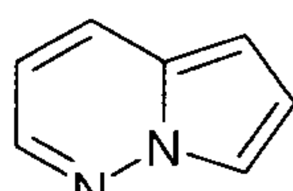
pyrrolo[1,2-b]pyridazine (pyrrolo[1,2-b]pyridazinyl)
