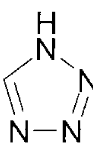
tetrazole (tetrazolyl)
