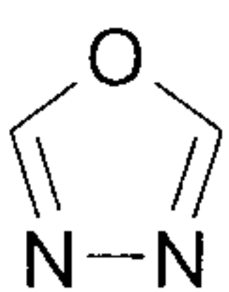
1-oxa-3,4-diazole (1-oxa-3,4-diazolyl)
