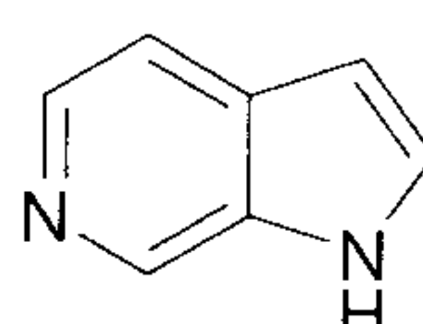
pyrrolo[2,3-c]pyridine (pyrrolo[2,3-c]pyridinyl)
