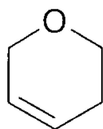
5,6-dihydro-2H-pyran (5,6-dihydro-2H-pyranyl)
