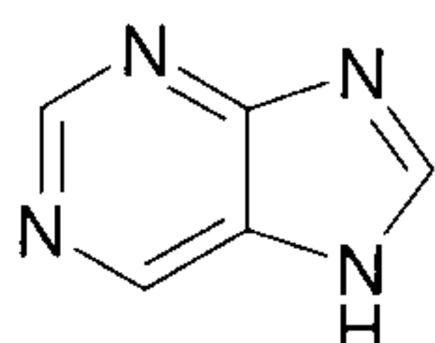
purine (purinyl)
