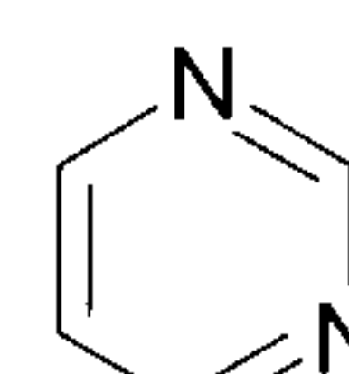
pyrimidine (pyrimidinyl)
