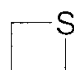
thiatane (thiatanyl)
