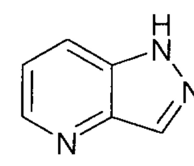
pyrazolo[4,3-d]pyridine (pyrazolo[4,3-d]pyridinyl)
