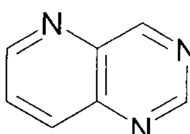
pyrido[3,2-d]pyrimidine (pyrido[3,2-d]pyrimidinyl)
