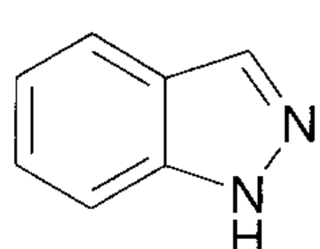
indazole (indazolyl)
