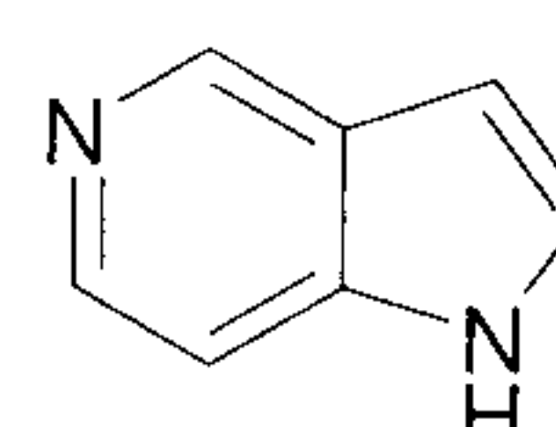
pyrrolo[3,2-c]pyridine (pyrrolo[3,2-c]pyridinyl)
