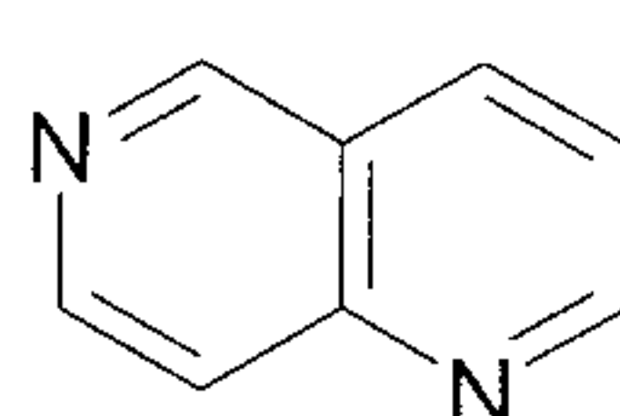
1,6-naphthyridine (1,6-naphthyridinyl)
