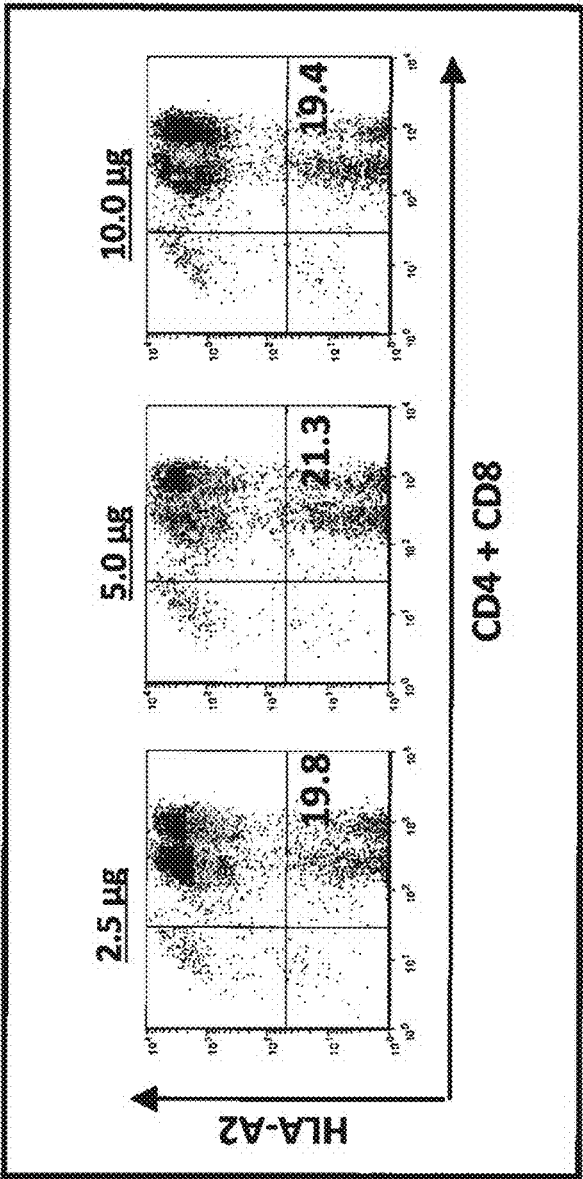
Figure 5A: standard
