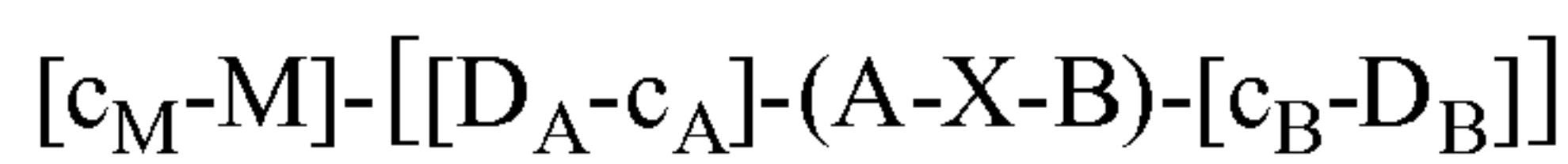
Formula I
