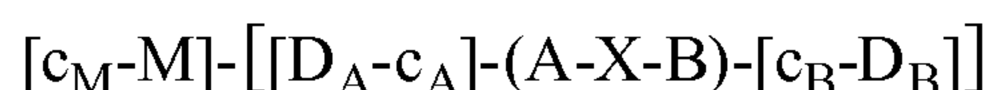
Formula I
