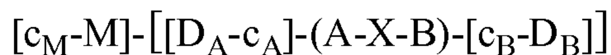
Formula I
