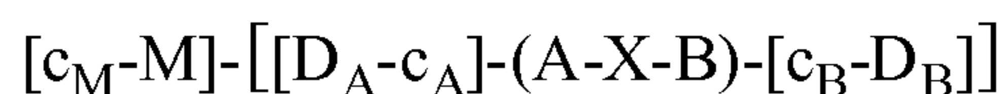
Formula I
