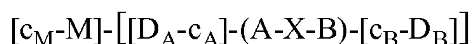
Formula I
