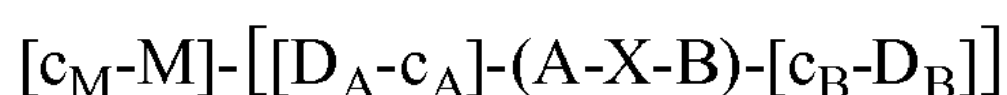
Formula I
