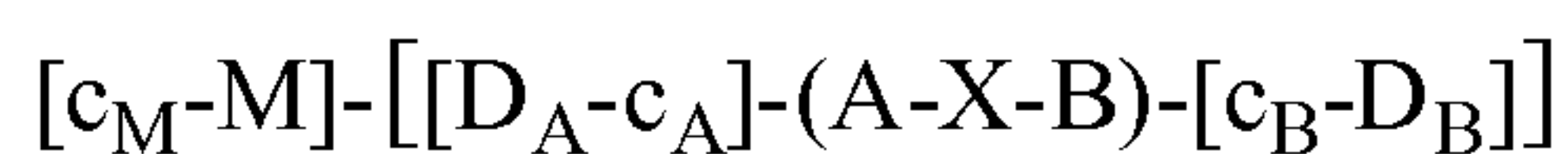
Formula I
