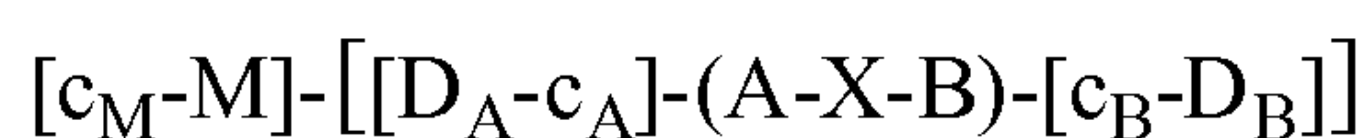
Formula I
