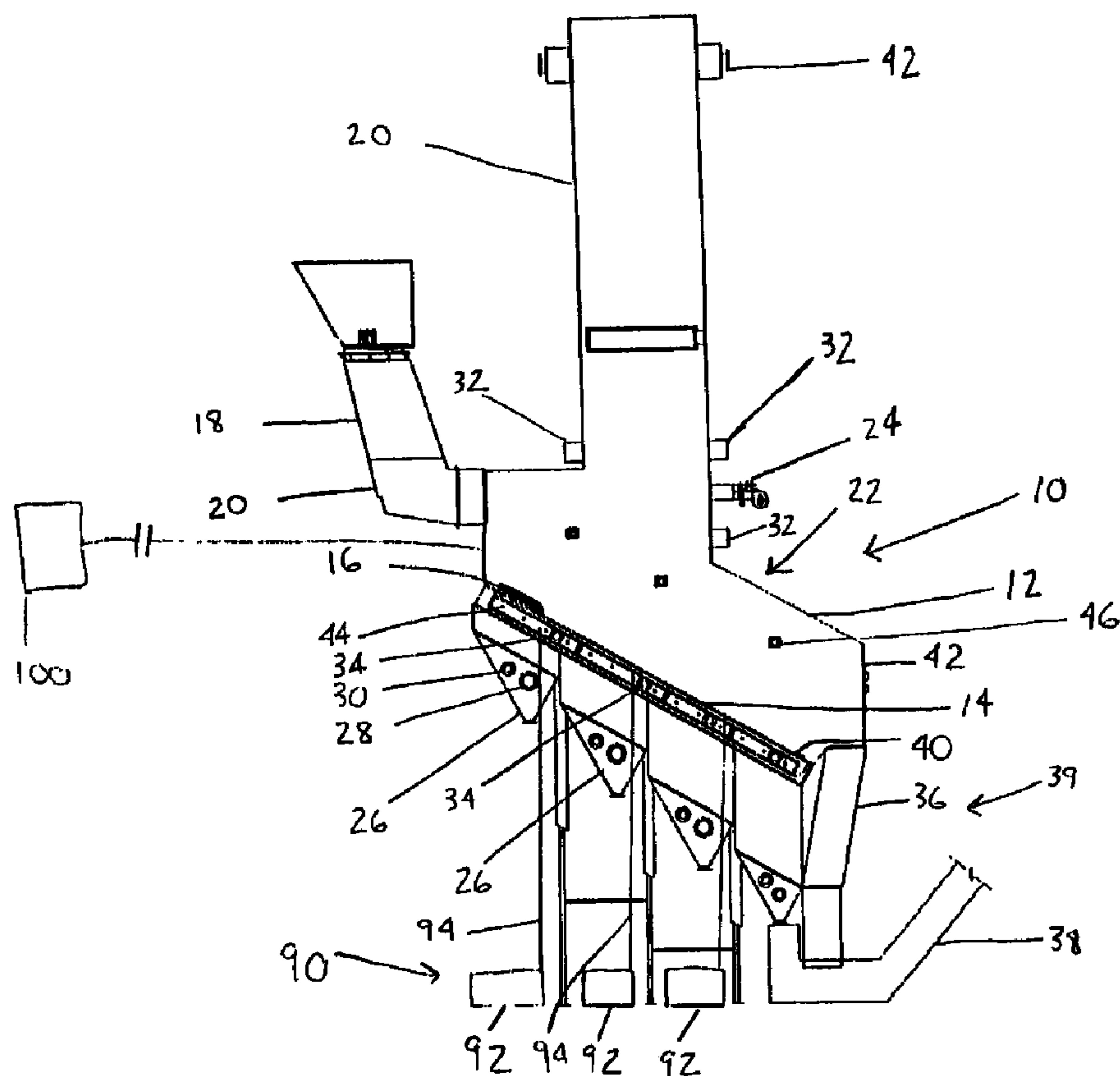
COMBUSTION SYSTEM ELEVATION VIEW
