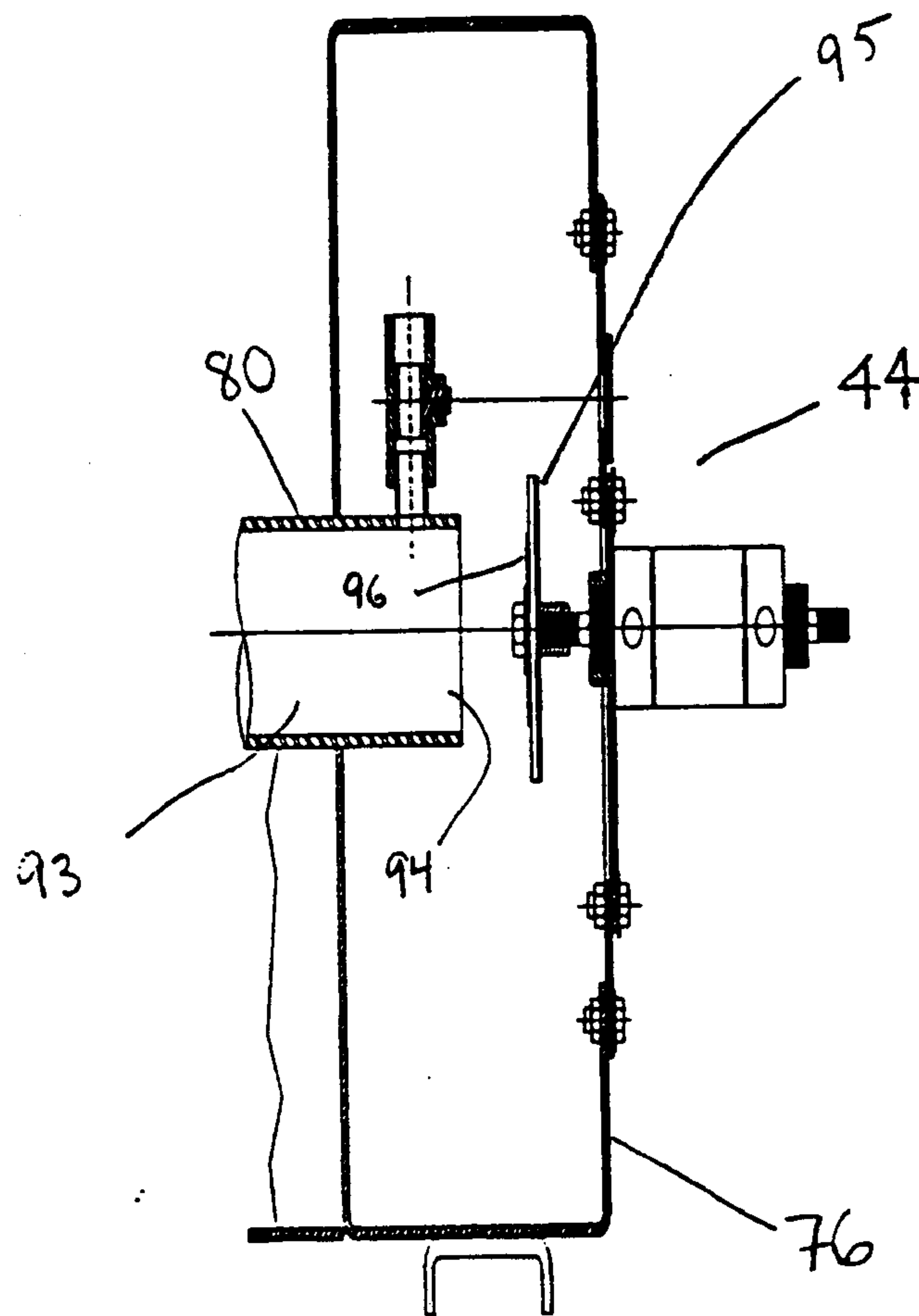
FIGURE 6: POPPET ASSEMBLY SIDE VIEW
