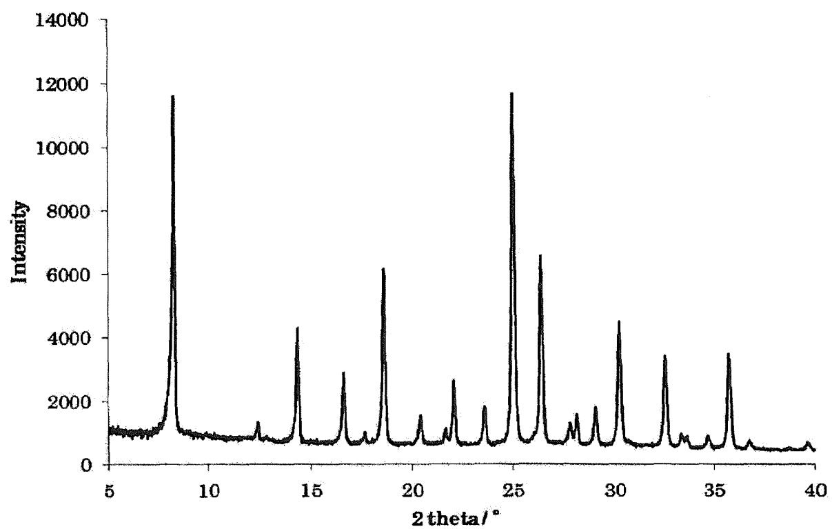
< XRD PATTERN OF ZEOLITE 9 >
