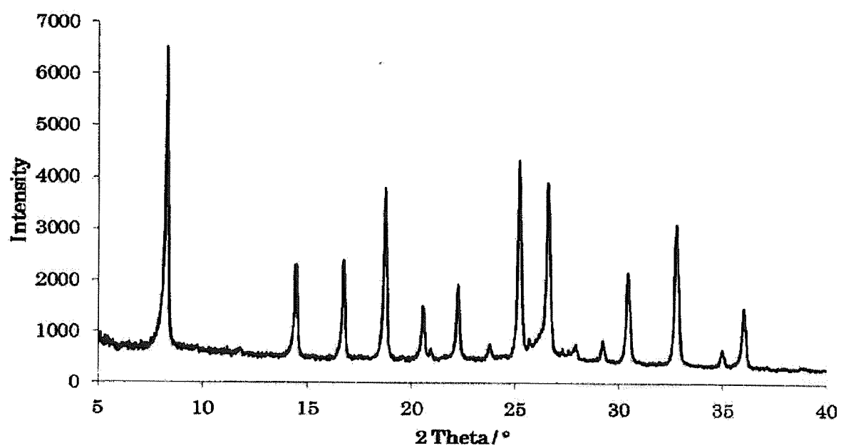
< XRD PATTERN OF ZEOLITE 6 >
