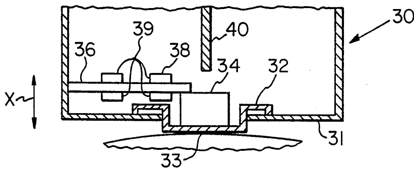
FIG. 4 PRIOR ART
