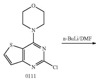
Scheme 9
