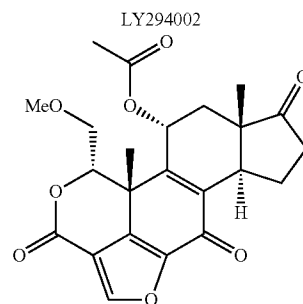
Wortmannin
