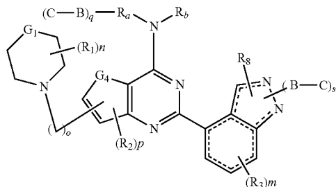
Formula XIII
