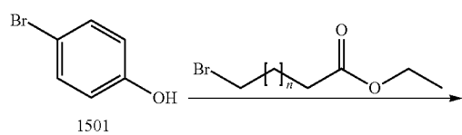
Scheme 15
