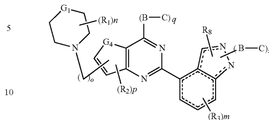
Formula IX
