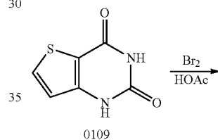
Scheme 10
