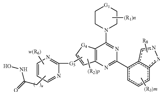
Formula XXV
