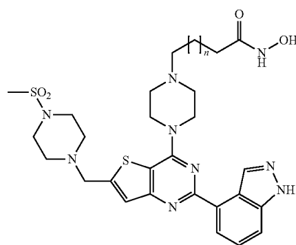
Scheme 9
