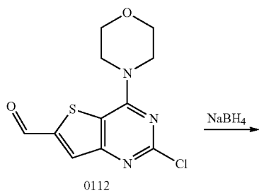
Scheme 5
