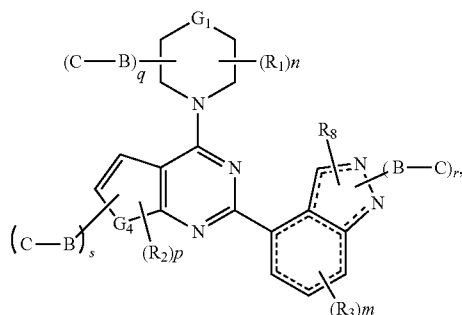
Formula VII
