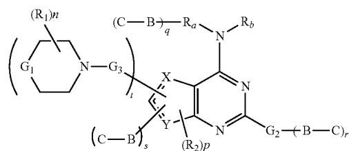
Formula I
