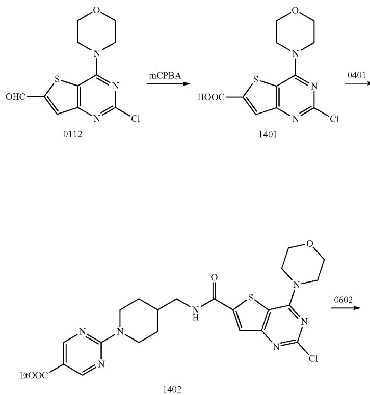
Scheme 14
