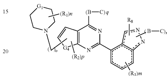
Formula IX
