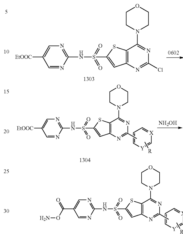
Scheme 14
