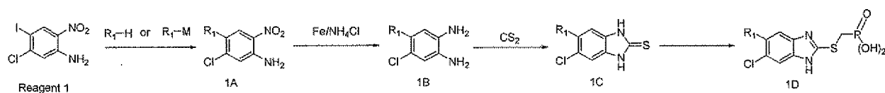
Scheme 1
