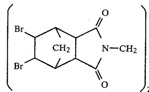
N 1 N 1 -ethylbis(dibromonorbornane- dicarboximide)
