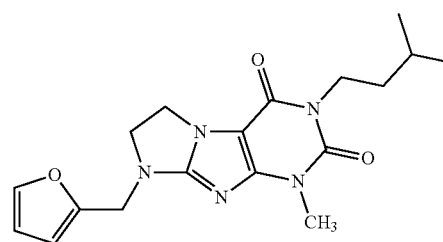
Compound I-56
