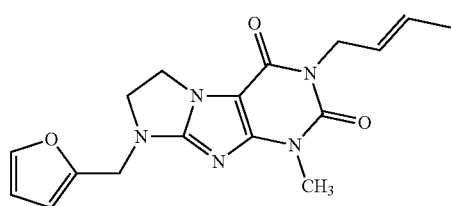
Compound I-53
