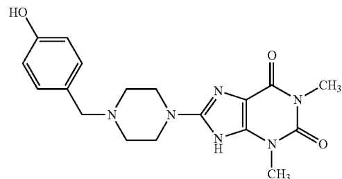
Compound B-7.1
