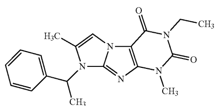
Compound I-31
