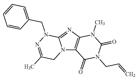
Compound V-17
