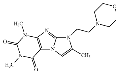
Compound A-3
