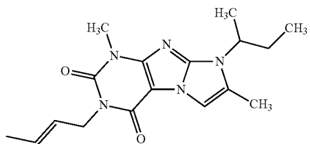
Compound I-4
