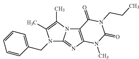
Compound I-35
