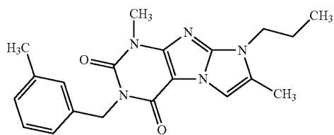
Compound I-24
