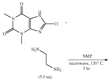
Scheme 11:
