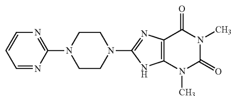
Compound B-6
