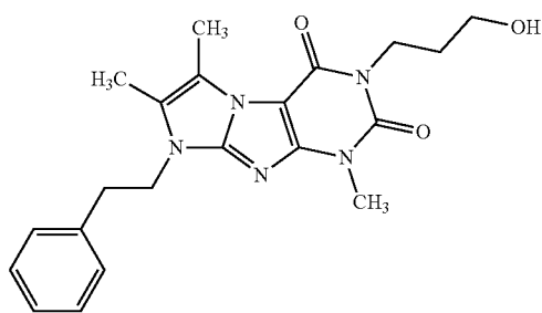
Compound I-48
