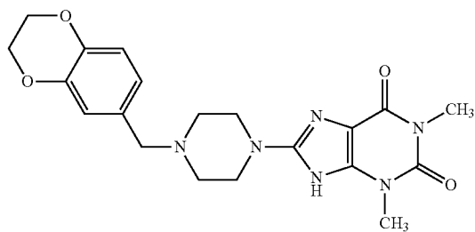
Compound B-7.8
