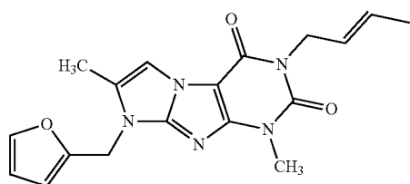
Compound I-53
