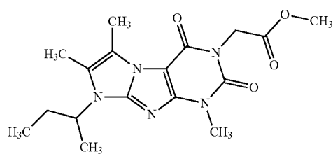
Compound I-50
