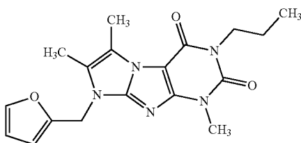
Compound I-33
