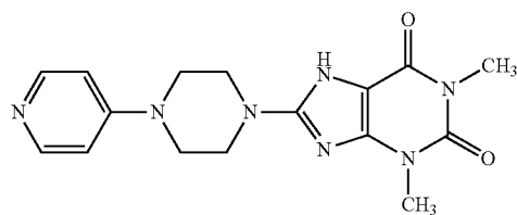
Compound B-4
