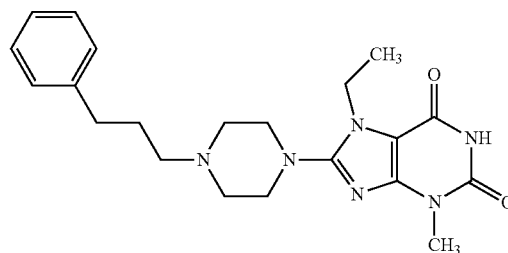
Compound III-4
