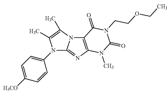
Compound I-46
