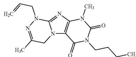
Compound V-7
