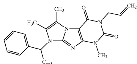
Compound I-44
