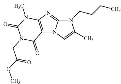
Compound I-41
