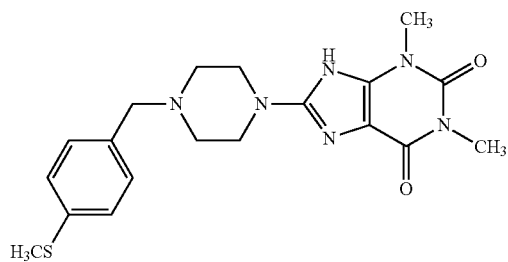
Compound B-7.4
