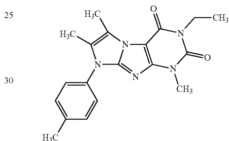
Compound I-2
