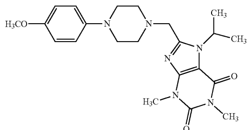
Compound III-6
