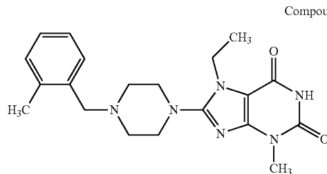
Compound III-4
