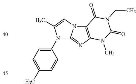
Compound I-3
