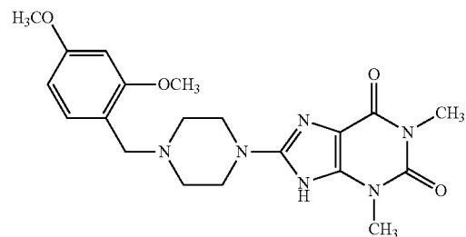
Compound B-7.12
