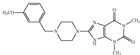
Compound B-7.11
