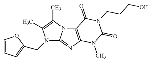
Compound I-47
