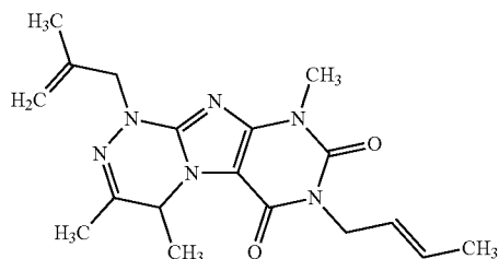
Compound V-21
