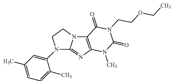
Compound I-41
