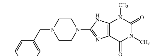
Compound B-7.2
