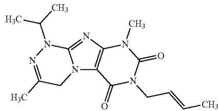
Compound V-18
