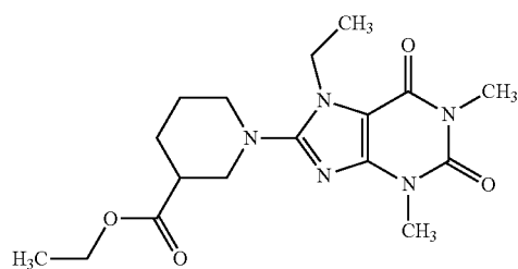
Compound III-6
