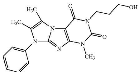
Compound I-41
