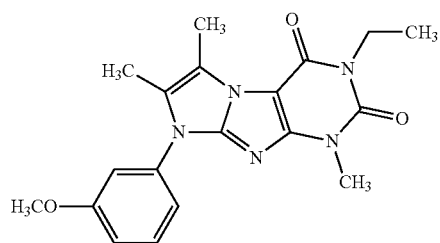
Compound I-29
