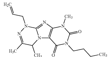
Compound V-10
