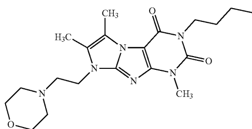
Compound I-52
