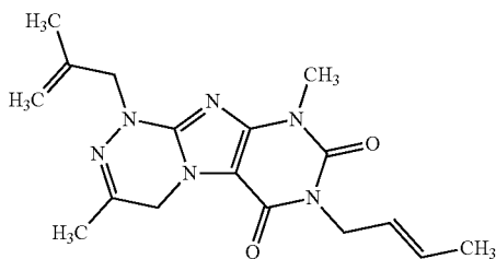
Compound V-3
