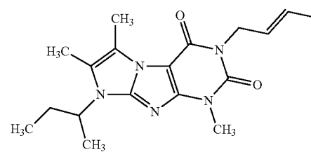
Compound I-57
