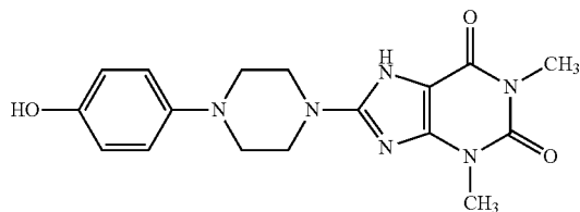
Compound B-7
