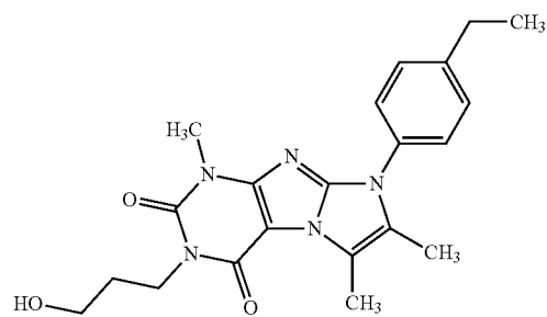
Compound I-34
