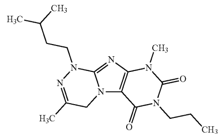
Compound V-10
