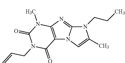
Compound I-1
