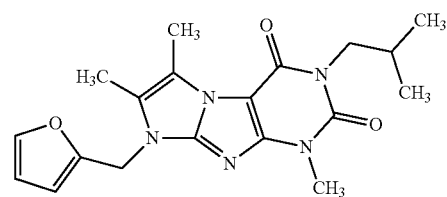
Compound I-45
