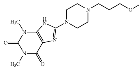
Compound B-7.19
