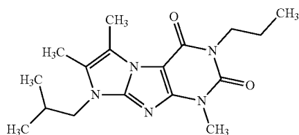
Compound I-31
