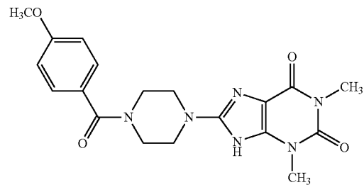
Compound B-7.17
