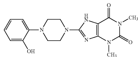
Compound III-3
