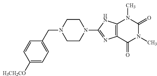
Compound B-7.3
