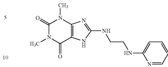
Compound B-14
