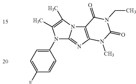
Compound I-1
