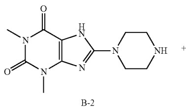
Scheme 7:
