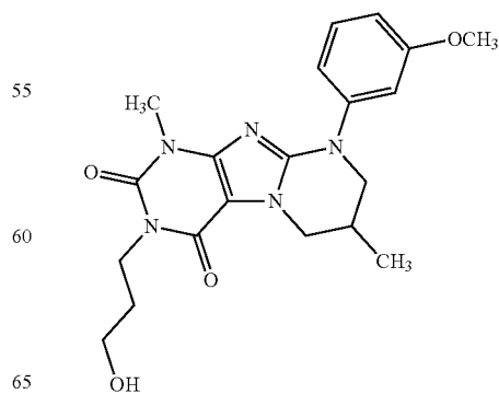
Compound IV-5
