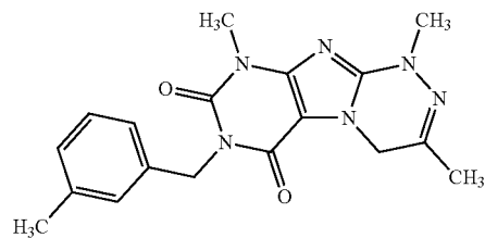
Compound V-9
