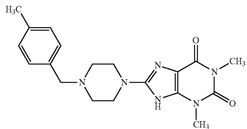
Compound B-7.5
