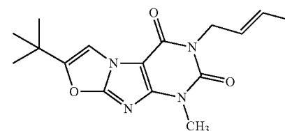
Compound A-8
