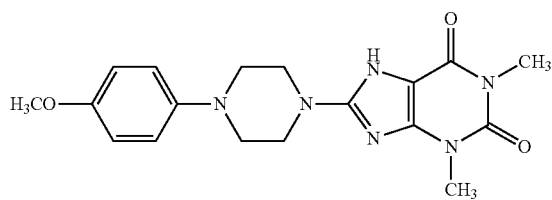
Compound B-7.19
