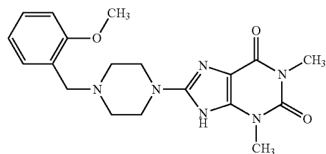
Compound B-7.9
