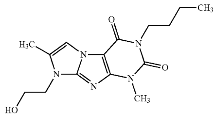
Compound I-29
