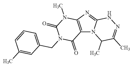
Compound V-11
