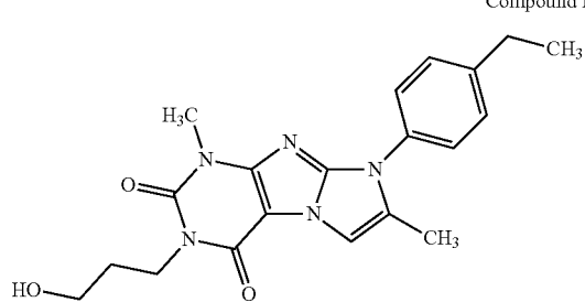
Compound I-43
