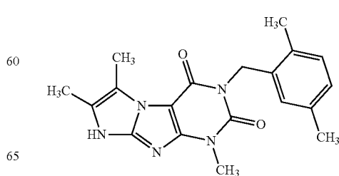
Compound I-11
