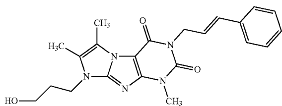
Compound I-51
