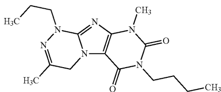
Compound V-4
