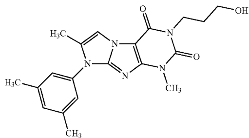
Compound I-40
