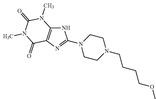
Compound B-7.20
