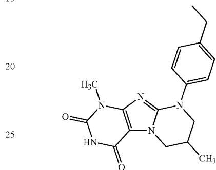
Compound IV-2
