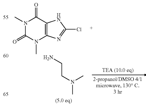
Scheme 9:
