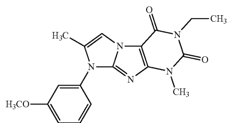
Compound I-35
