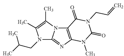
Compound I-39
