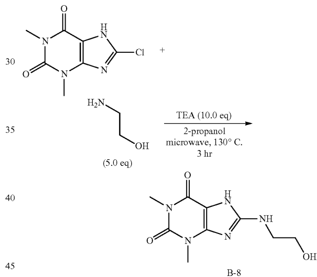
Scheme 8:
