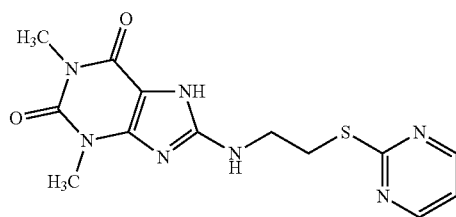
Compound B-12
