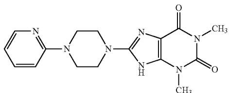
Compound B-4
