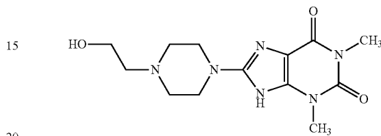
Compound B-15
