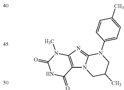
Compound IV-4
