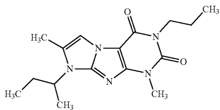
Compound I-38
