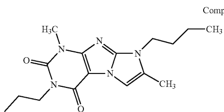
Compound I-3
