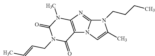
Compound I-28
