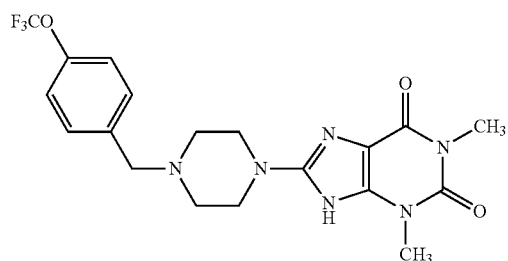
Compound B-7.6
