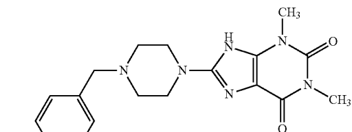
Compound B-7.1
