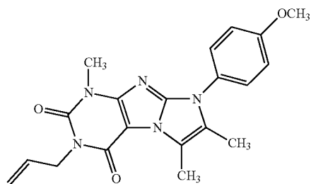
Compound I-27
