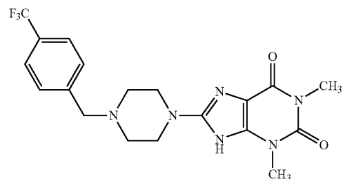
Compound B-7.8
