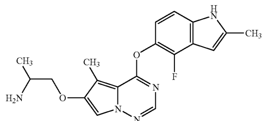
2-[4-(4-Fluoro-2-methyl-1H-indol-5-yloxy)-5-methylpyrrolo[2,1-f][1,2,4]triazin-6-yloxy]-1-methylethylamine
