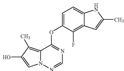
4-(4-Fluoro-2-methyl-1H-indol-5-yloxy)-5-methylpyrrolo[2,1-f][1,2,4]triazine-6-ol
