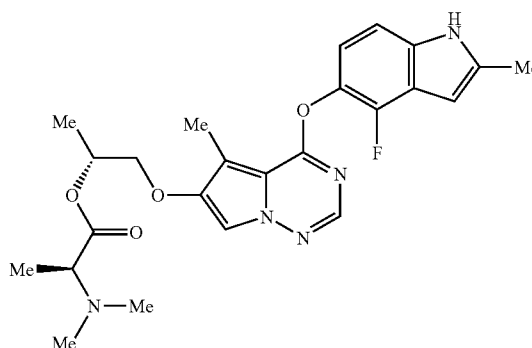
[(1R,2S)-2-Dimethylaminopropionic acid-[2-[4-(4-fluoro-2-methyl-1H-indol-5-yloxy)-5-methylpyrrolo[2,1-f][1,2,4]triazin-6-yloxy]]-1-methylethyl ester
