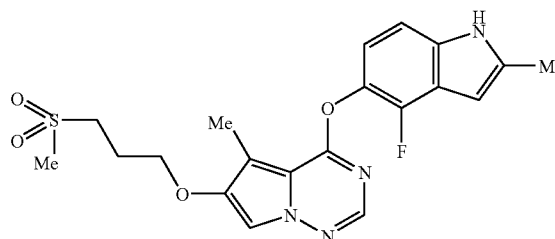
4-(4-Fluoro-2-methyl-1H-indol-5-yloxy)-6-(3-methanesulfonyl-propoxy)-5-methylpyrrolo[2,1-f][1,2,4]triazine
