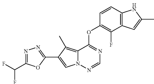
6-(5-Difluoromethyl-[1,3,4]oxadiazol-2-yl)-4-(4-fluoro-2-methyl-1H-indol-5-yloxy)-5-methylpyrrolo[2,1-f][1,2,4]triazine
