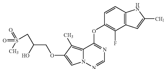
1-[4-(4-Fluoro-2-methyl-1H-indol-5-yloxy)-5-methylpyrrolo[2,1-f][1,2,4]triazin-6-yloxy]-3-methanesulfonylpropan-2-ol
