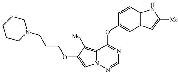
5-Methyl-4-(2-methyl-1H-indol-5-yloxy)-6-(3-piperidin-1-ylpropoxy)-pyrrolo[2,1-f[1,2,4]triazine
