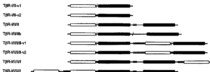
Single-chain trap
