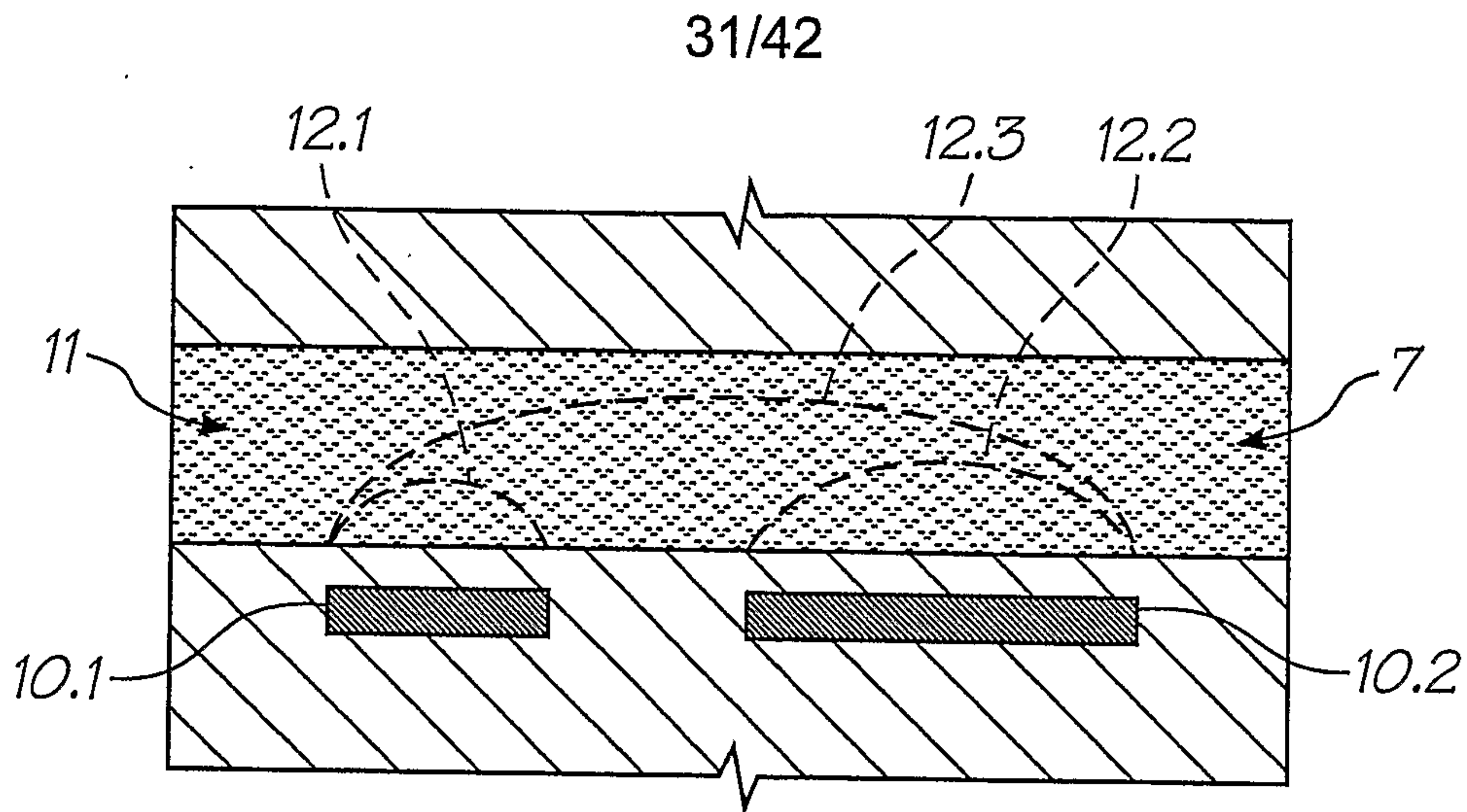
FIG. 52 (PRIOR ART)
