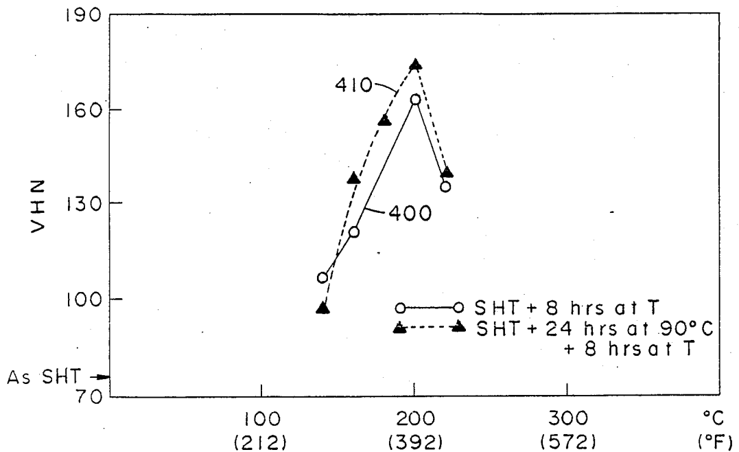
HARDENING RESPONSE OF ALLOY 2090
