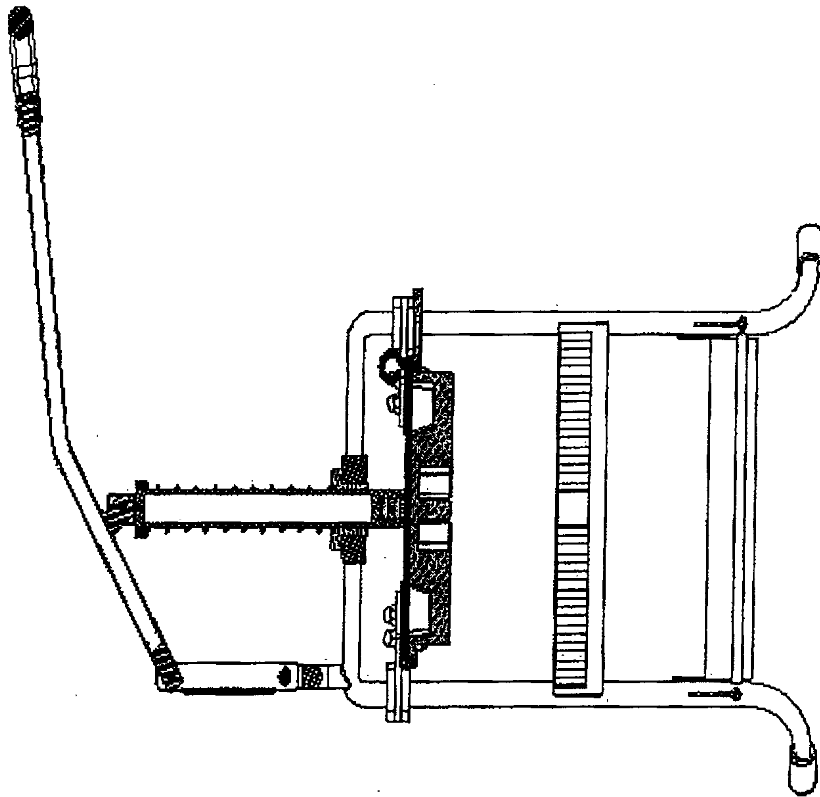
SECTION AA
