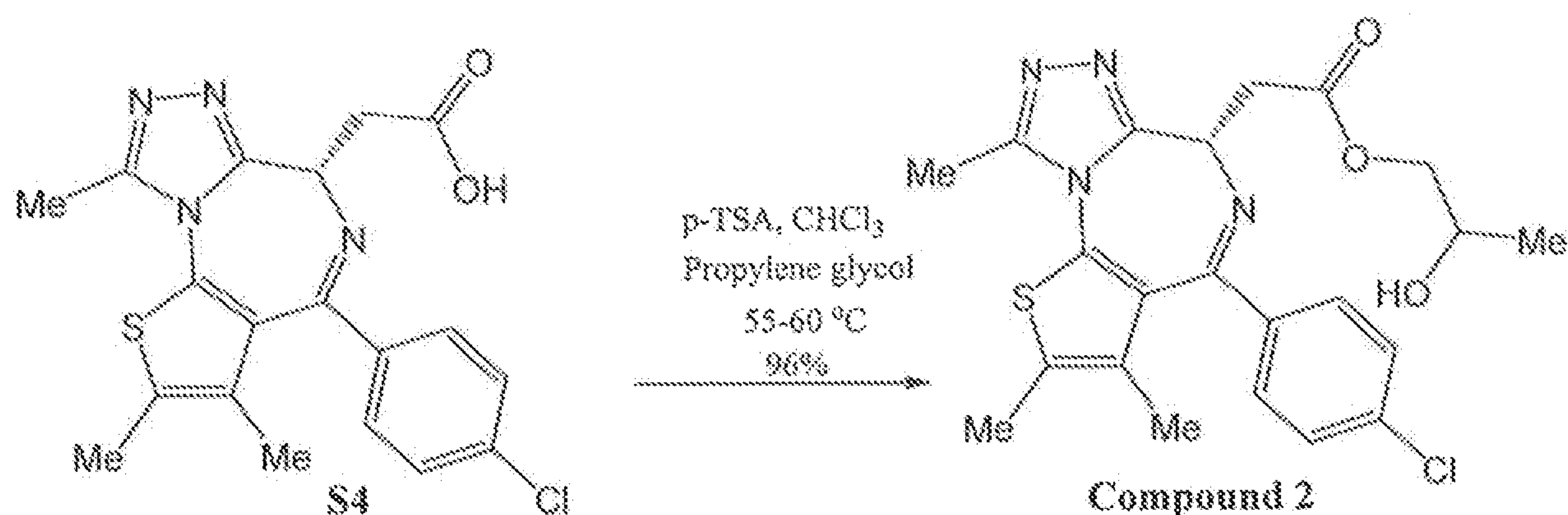
Scheme S2. Synthesis of Compound 2-Example 2
