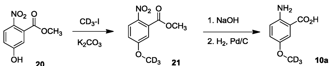
Scheme 2. Synthesis of Intermediate 10a , wherein R^1 = CD_3
