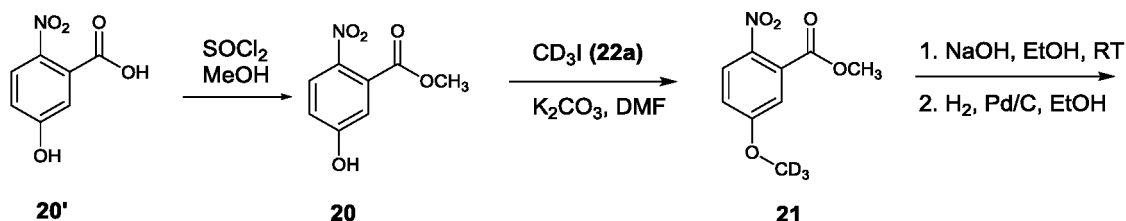
Scheme 4: Preparation of Compound 104
