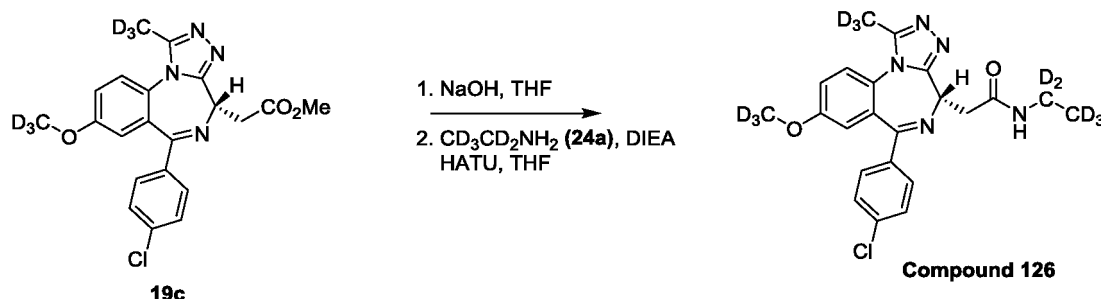
Scheme 10: Preparation of Compound 126
