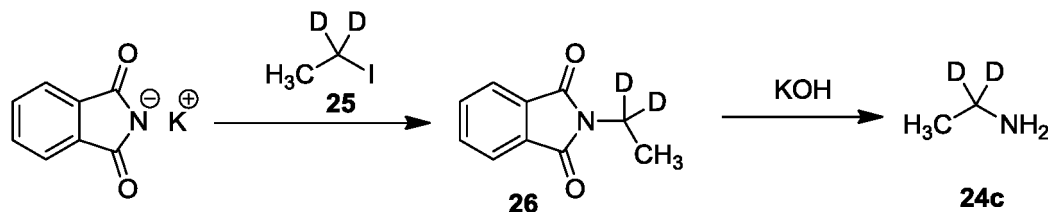
Scheme 3. Synthesis of 24c
