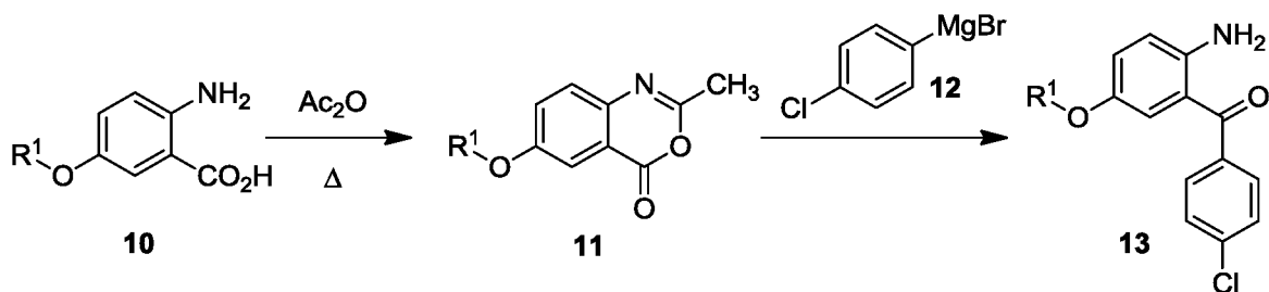
Scheme 1. Synthesis of Compounds of Formula I
