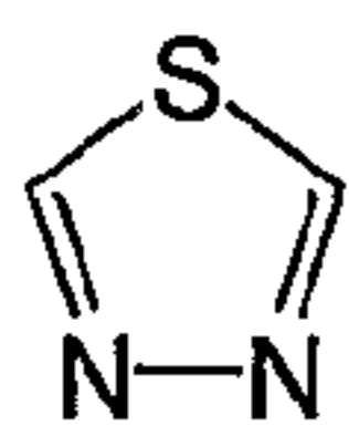
1-thia-3,4-diazole (1-thia-3,4-diazolyl)
