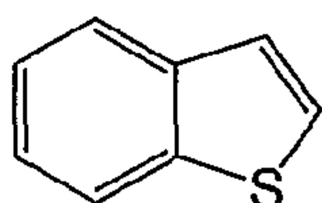
benzothiophene (benzothiophenyl)
