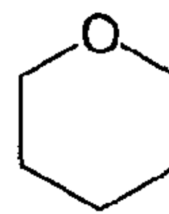
tetrahydropyran (tetrahydropyranyl)
