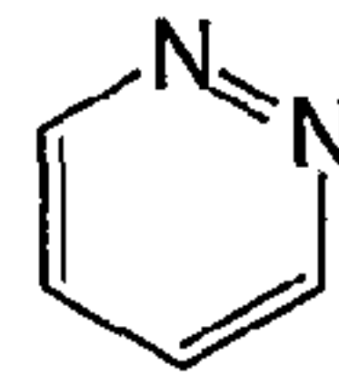
pyridazine (pyridazinyl)
