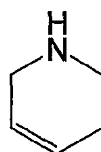
1,2,5,6-tetrahydropyridine (1,2,5,6-tetrahydropyridinyl)
