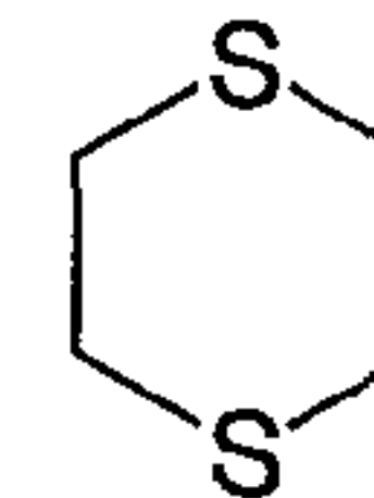
1,4-dithiane (1,4-dithianyl)
