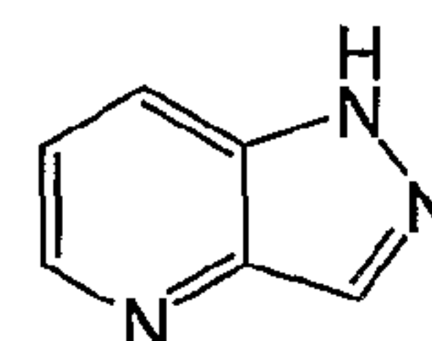
pyrazolo[4,3-d]pyridine (pyrazolo[4,3-d]pyridinyl)
