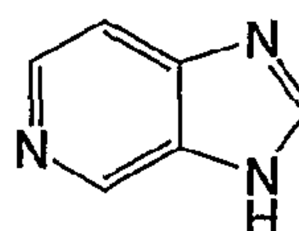
imidazo[4,5-c]pyridine (imidazo[4,5-c]pyridinyl)
