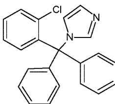
Clotrimazole
