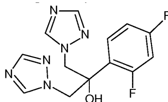
Fluconazole
