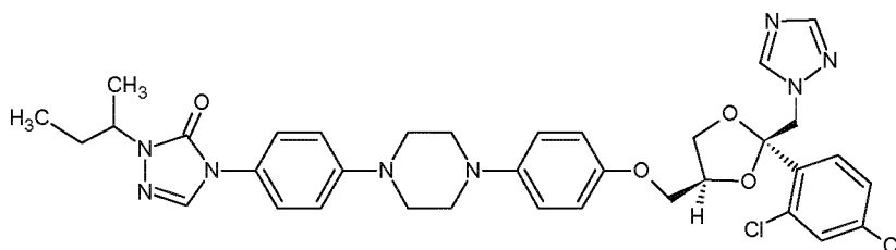
Itraconazole
