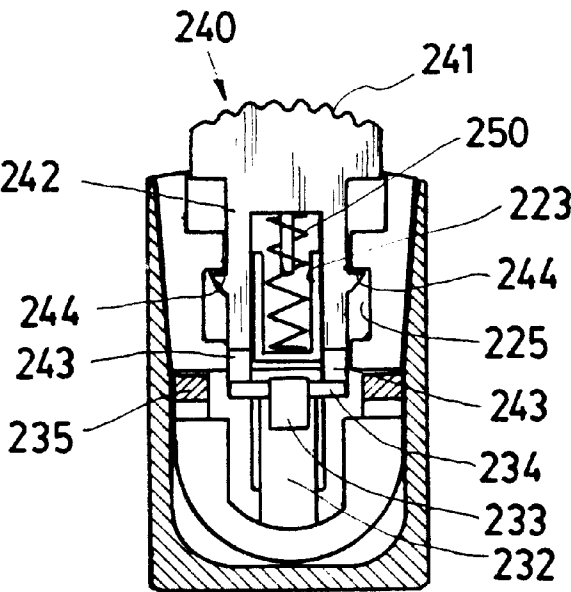
B-B Sec. FIG. 6
