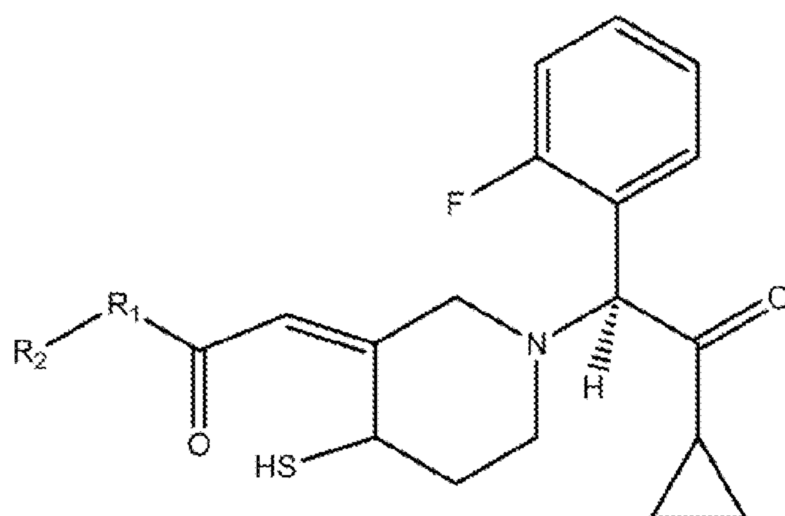
Formula IIa
