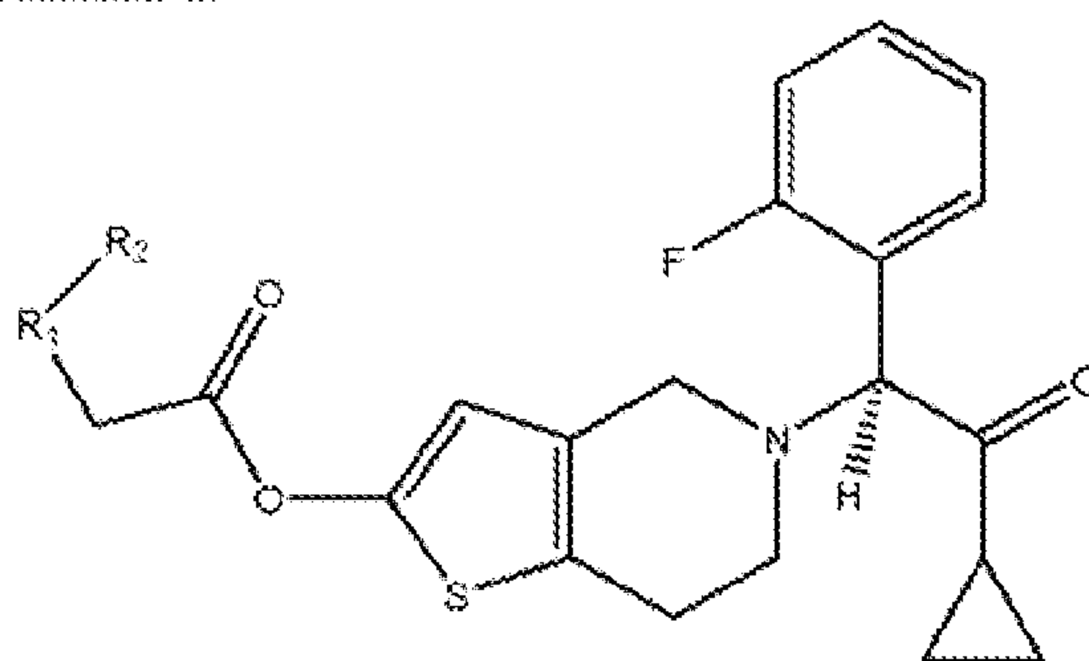
Formula II
