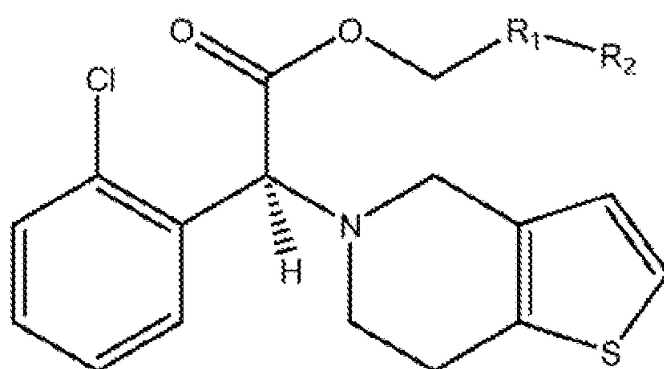
Formula I
