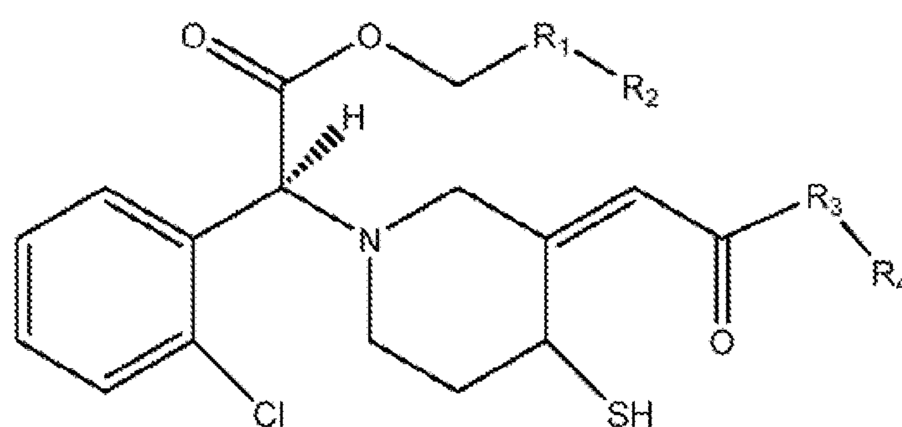
formula Ia
