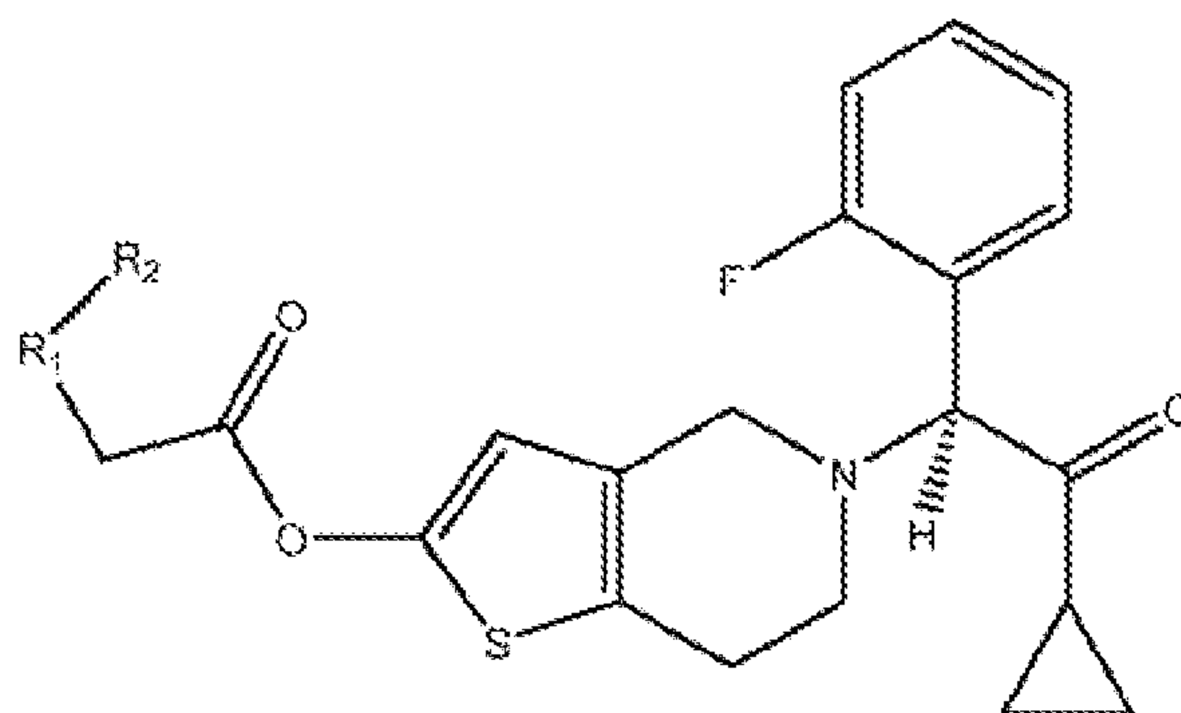
Formula II
