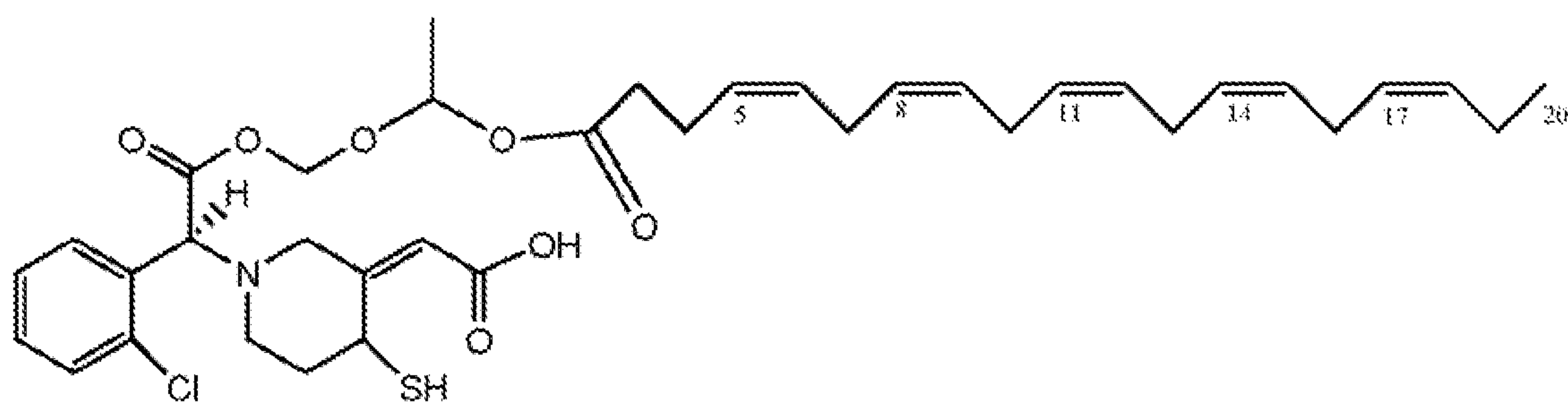
(1a-1)
