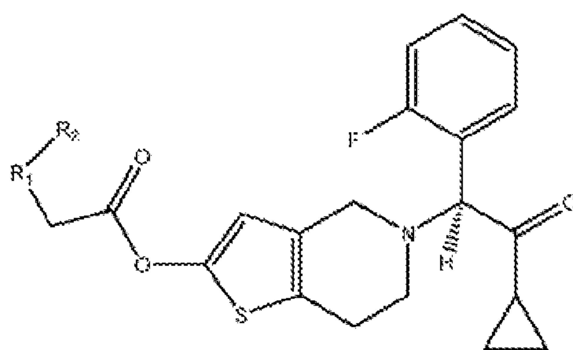
Formula II
