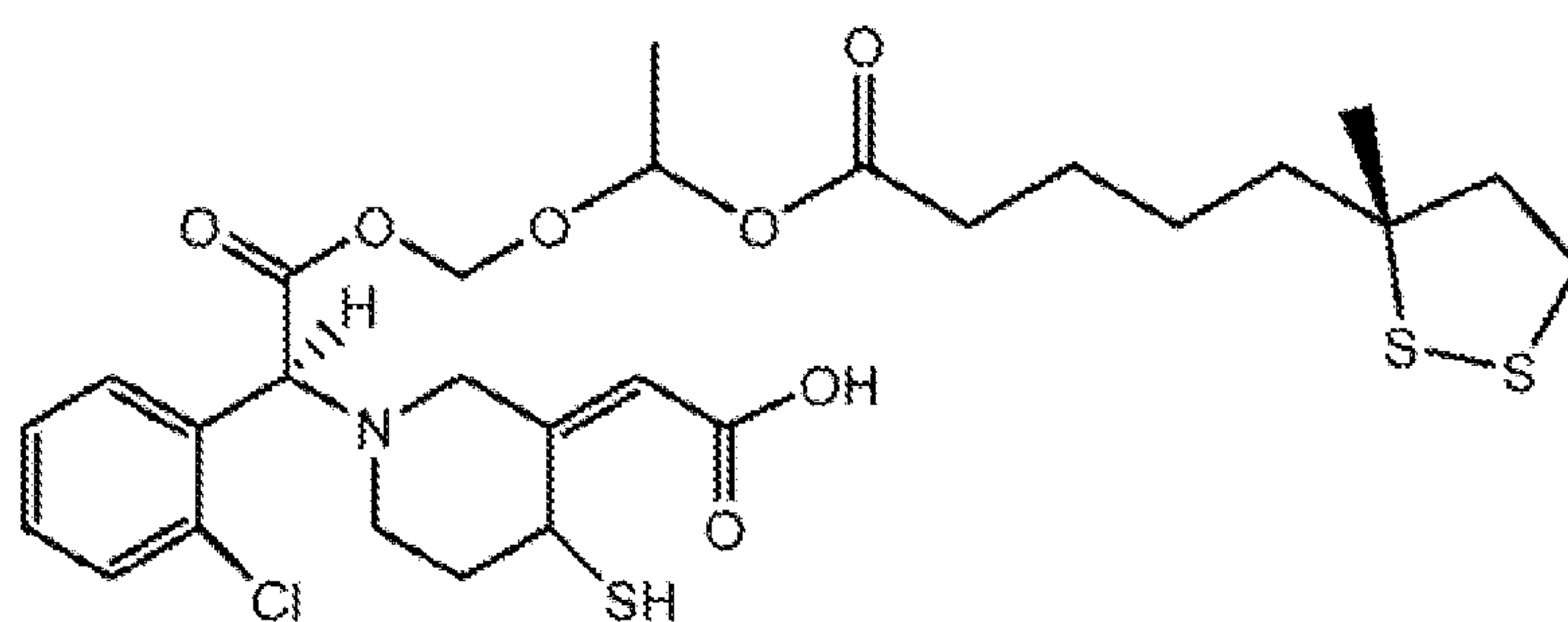
(1a-1)
