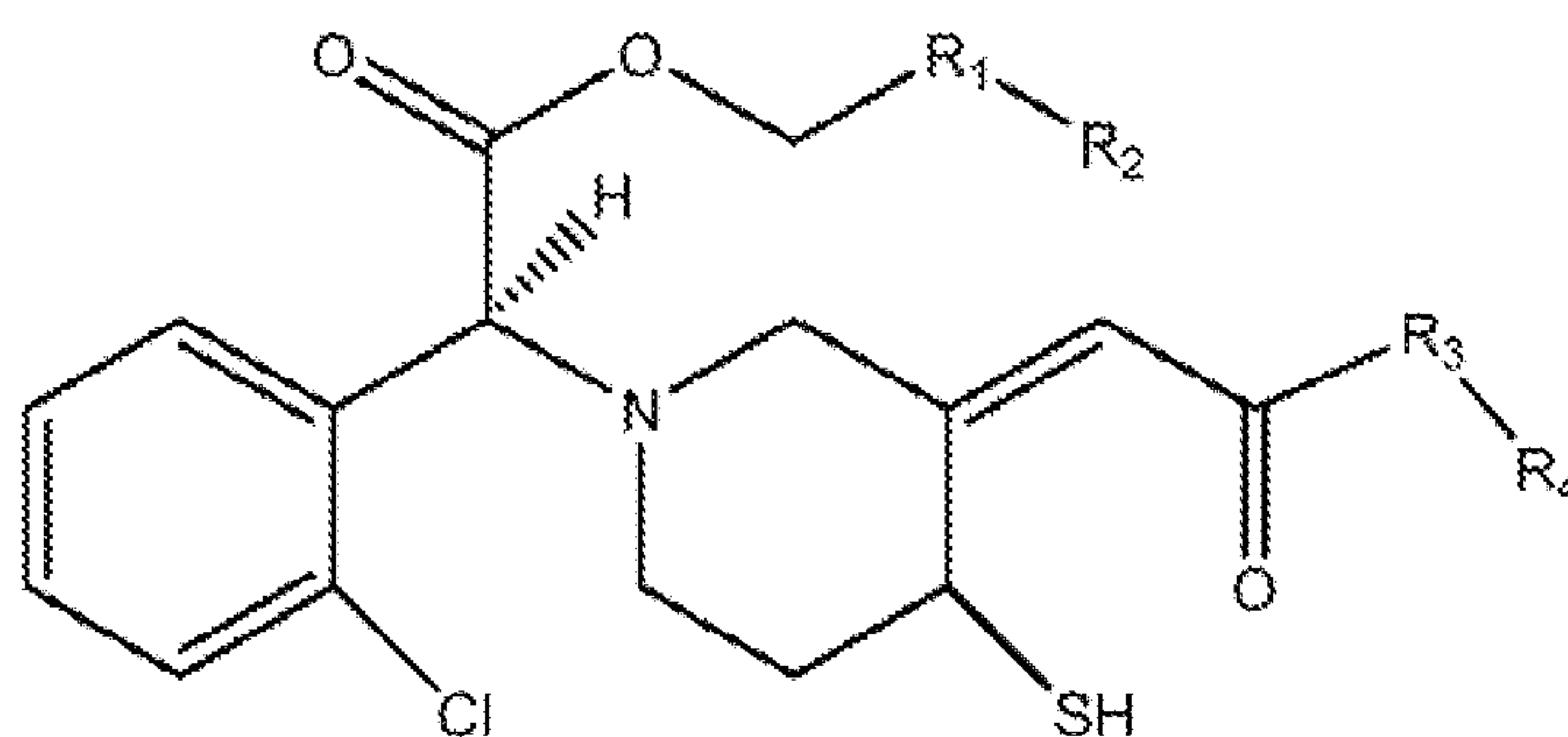
Formula Ia
