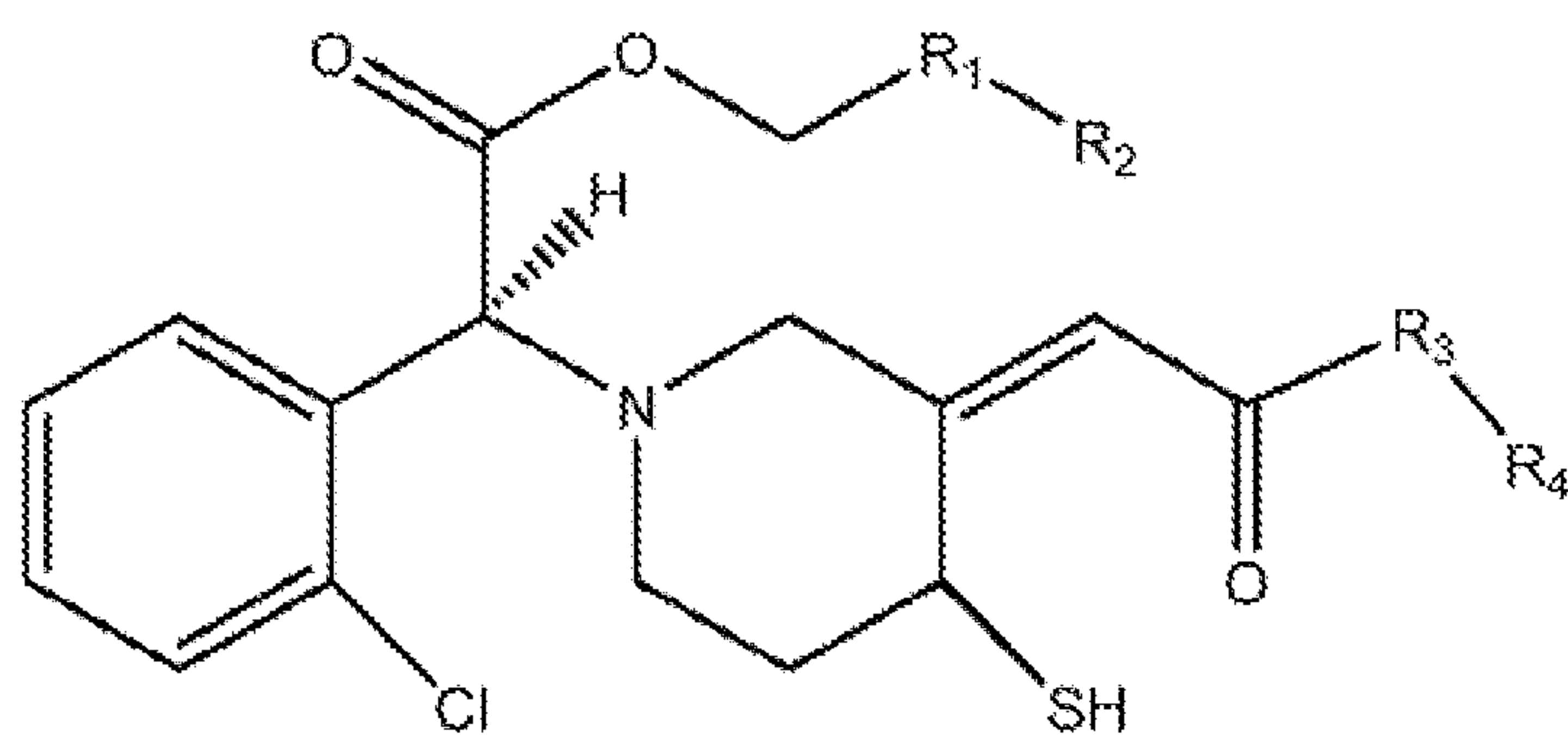
formula Ia
