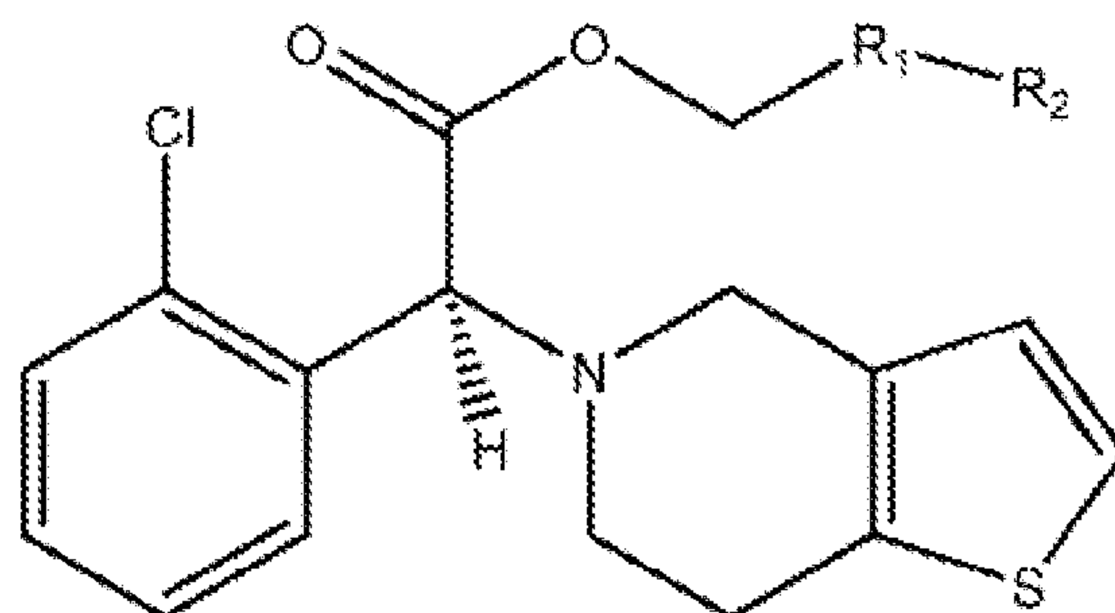
Formula I
