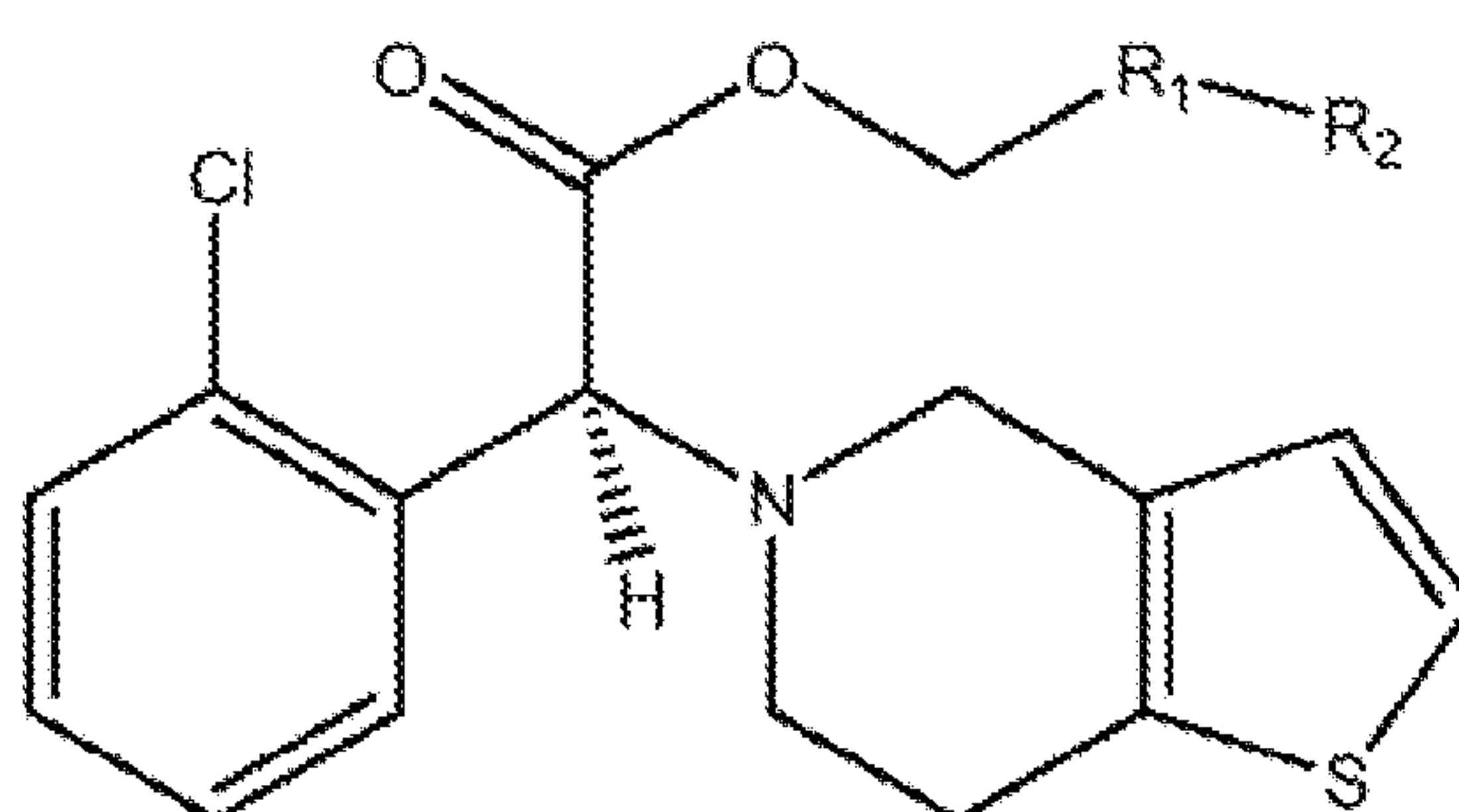
Formula I
