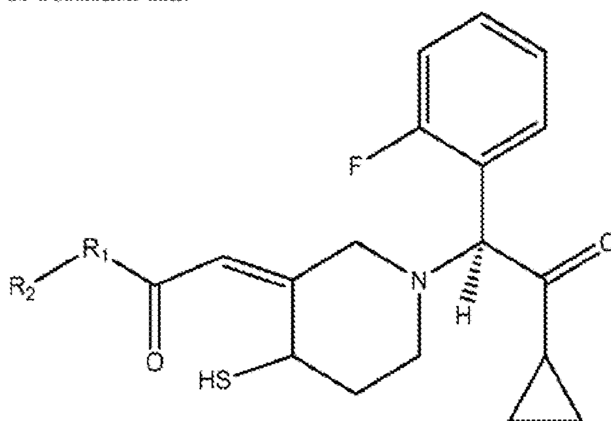
Formula IIa
