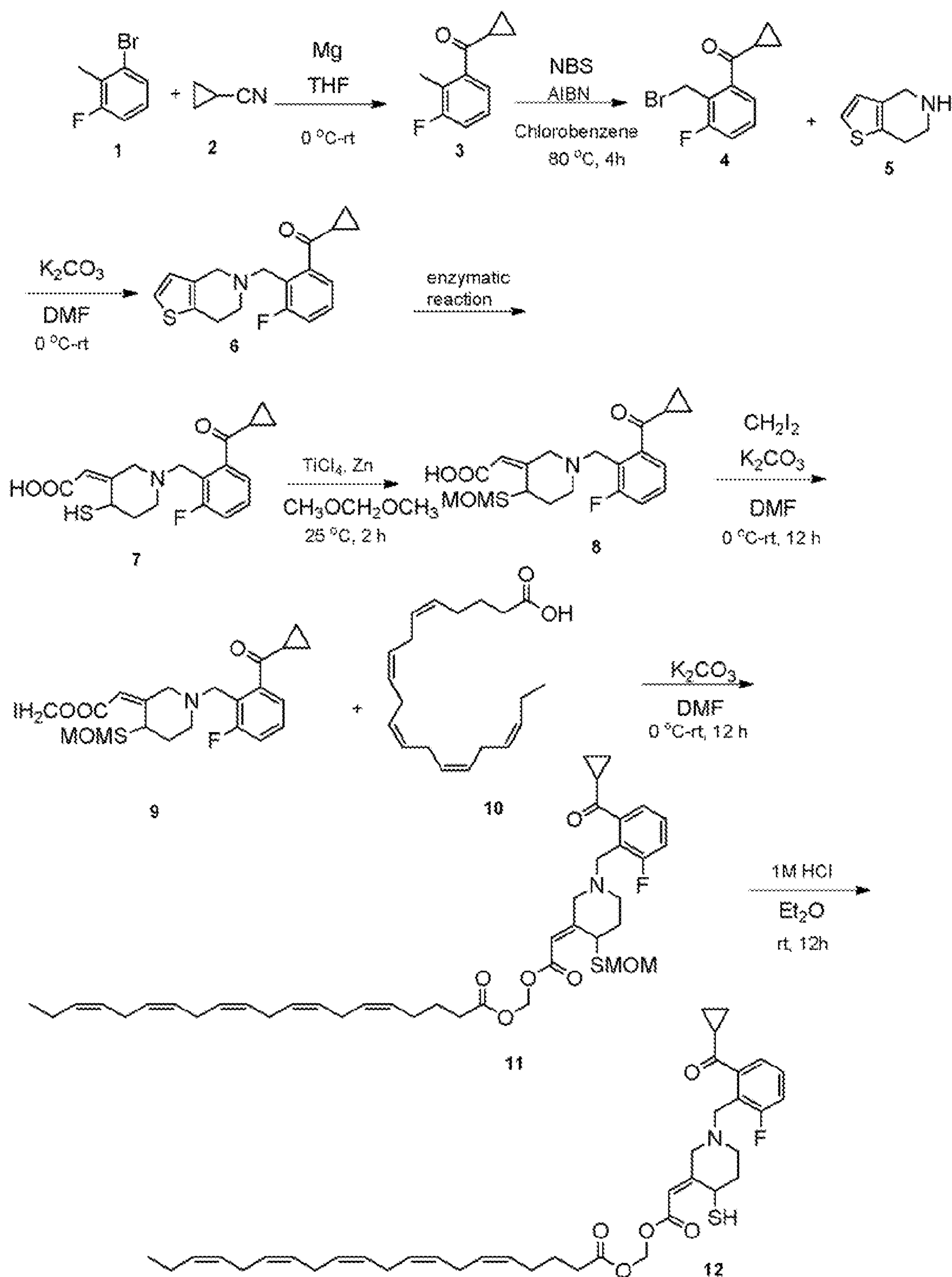
Scheme – 2:
