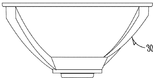
BOTTOM VIEW Fig. 7B
