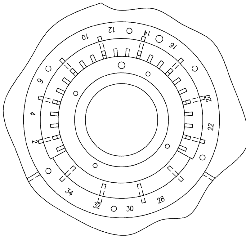
SECTION J-J Fig. 5N
