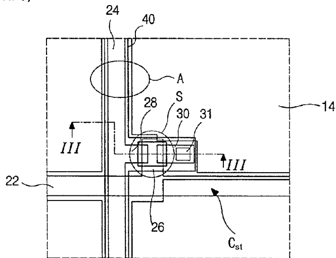
FIG.2 (Related Art)
