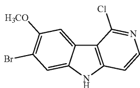
7-bromo-1-chloro-8-methoxy-5H-pyrido[4,3-b]indole
