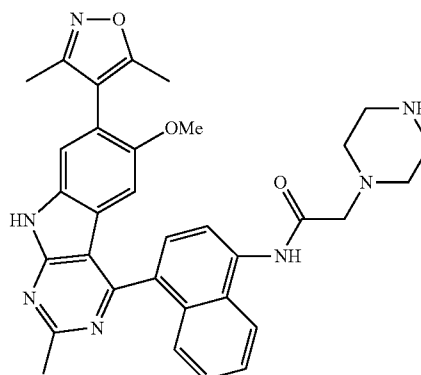
N-(4-(7-(3,5-Dimethylisoxazol-4-yl)-6-methoxy-2-methyl-9H-pyrimido[4,5-b]indol-4-yl)naphthalen-1-yl)-2-(piperazin-1-yl)acetamide
