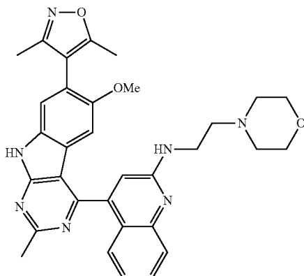
4-(7-(3,5-Dimethylisoxazol-4-yl)-6-methoxy-2-methyl-9H-pyrimido[4,5-b]indol-4-yl)-N-(2-morpholinoethyl)quinolin-2-amine
