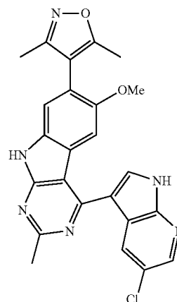
4-(4-(5-Chloro-1H-pyrrolo[2,3-b]pyridin-3-yl)-6-methoxy-2-methyl-9H-pyrimido[4,5-b]indol-7-yl)-3,5-dimethylisoxazole
