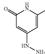
4-Hydrazinyl-6-methylpyridin-2(1H)-one
