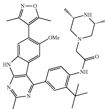
N-(2-(tert-Butyl)-4-(7-(3,5-dimethylisoxazol-4-yl)-6-methoxy-2-methyl-9H-pyrimido[4,5-b]indol-4-yl)phenyl)-2-((3R,5S)-3,5-dimethylpiperazin-1-yl)acetamide
