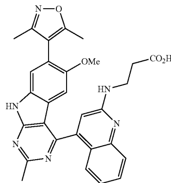
3-((4-(7-(3,5-Dimethylisoxazol-4-yl)-6-methoxy-2-methyl-9H-pyrimido[4,5-b]indol-4-yl)-N-(3-(4-methylpiperazin-1-yl)propyl)quinolin-2-yl)amino)propanoic acid
