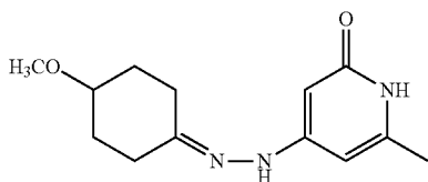
4-(2-(4-Methoxycyclohexylidene)hydrazinyl)-6-methylpyridin-2(1H)-one
