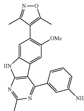
3-(7-(3,5-Dimethylisoxazol-4-yl)-6-methoxy-2-methyl-9H-pyrimido[4,5-b]indol-4-yl)aniline
