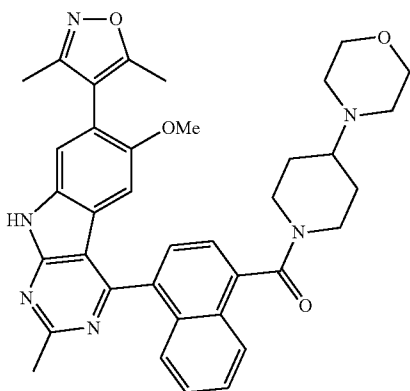
(4-(7-(3,5-Dimethylisoxazol-4-yl)-6-methoxy-2-methyl-9H-pyrimido[4,5-b]indol-4-yl)naphthalen-1-yl)(4-morpholinopiperidin-1-yl)methanone
