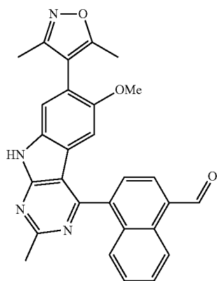
4-(7-(3,5-Dimethylisoxazol-4-yl)-6-methoxy-2-methyl-9H-pyrimido[4,5-b]indol-4-yl)-1-naphthaldehyde (CE 194)
