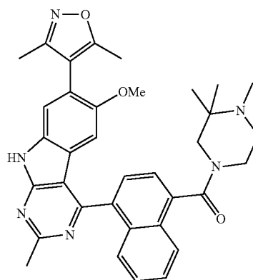
(4-(7-(3,5-Dimethylisoxazol-4-yl)-6-methoxy-2-methyl-9H-pyrimido[4,5-b]indol-4-yl)naphthalen-1-yl)(3,3,4-trimethylpiperazine-1-yl)methanone
