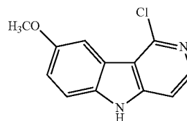
1-chloro-8-methoxy-5H-pyrido[4,3-b]indole
