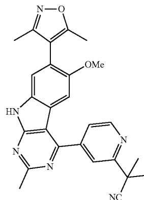
2-(4-(7-(3,5-Dimethylisoxazol-4-yl)-6-methoxy-2-methyl-9H-pyrimido[4,5-b]indol-4-yl)pyridin-2-yl)-2-methylpropanenitrile
