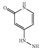
4-hydrazinylpyridin-2(1H)-one
