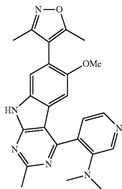
2-(7-(3,5-Dimethylisoxazol-4-yl)-6-methoxy-2-methyl-9H-pyrimido[4,5-b]indol-4-yl)-N,N-dimethylaniline
