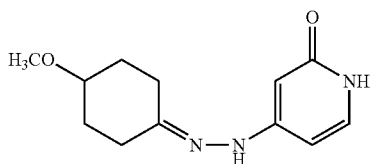
4-(2-(4-methoxycyclohexylidene)hydrazinyl)pyridin-2(1H)-one
