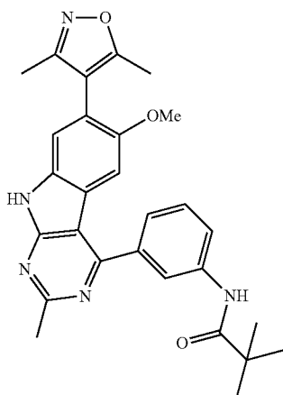
N-(3-(7-(3,5-Dimethylisoxazol-4-yl)-6-methoxy-2-methyl-9H-pyrimido[4,5-b]indol-4-yl)phenyl)pivalamide
