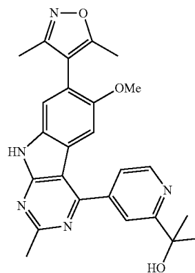
2-(4-(7-(3,5-Dimethylisoxazol-4-yl)-6-methoxy-2-methyl-9H-pyrimido[4,5-b]indol-4-yl)pyridin-2-yl)propan-2-ol
