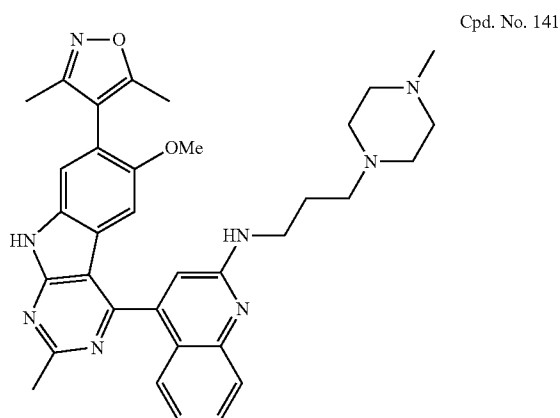
4-(7-(3,5-Dimethylisoxazol-4-yl)-6-methoxy-2-methyl-9H-pyrimido[4,5-b]indol-4-yl)-N-(3-(4-methylpiperazin-1-yl)propyl)quinolin-2-amine
