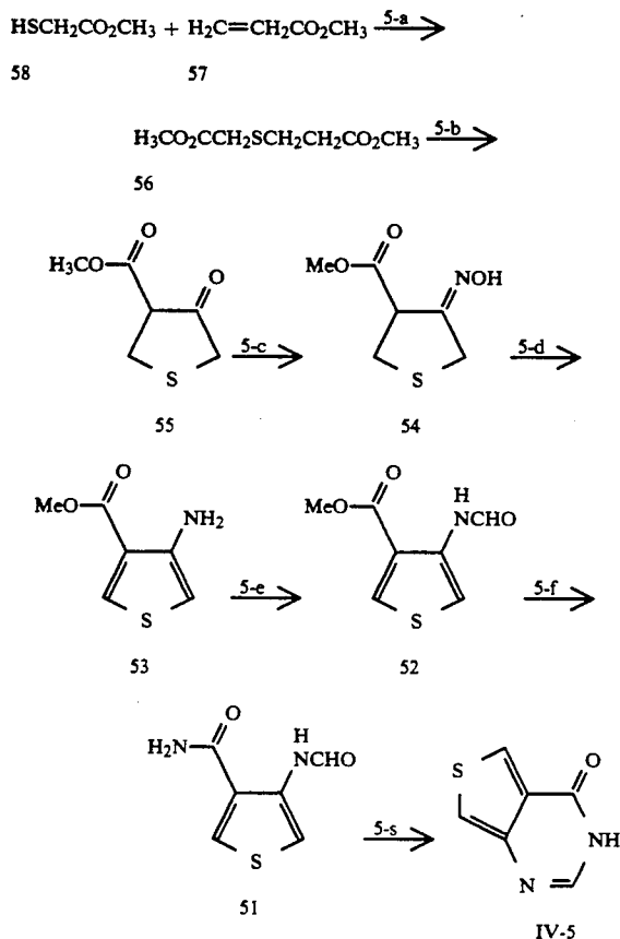
Scheme 5
