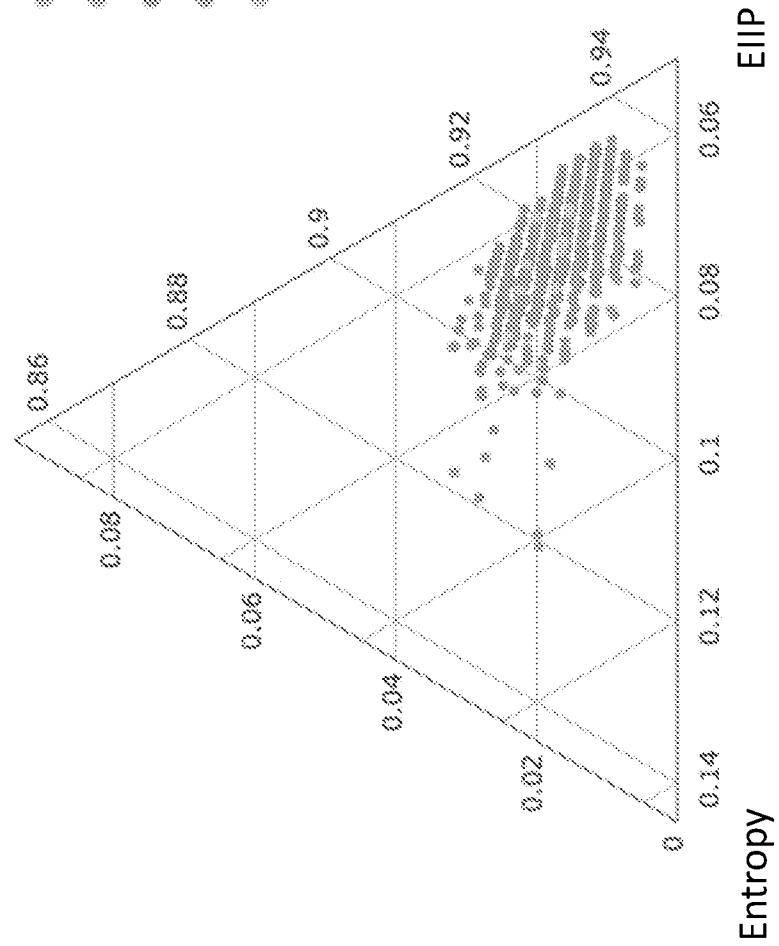
GC Content
