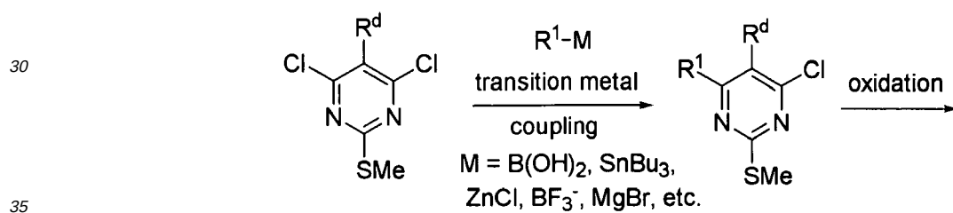
Scheme 2.d
