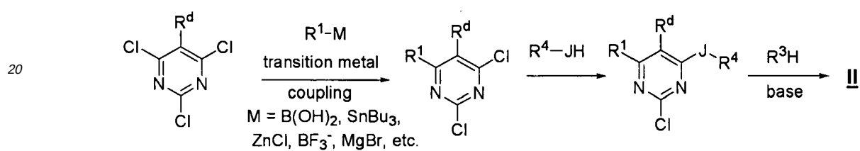
Scheme 2.c
