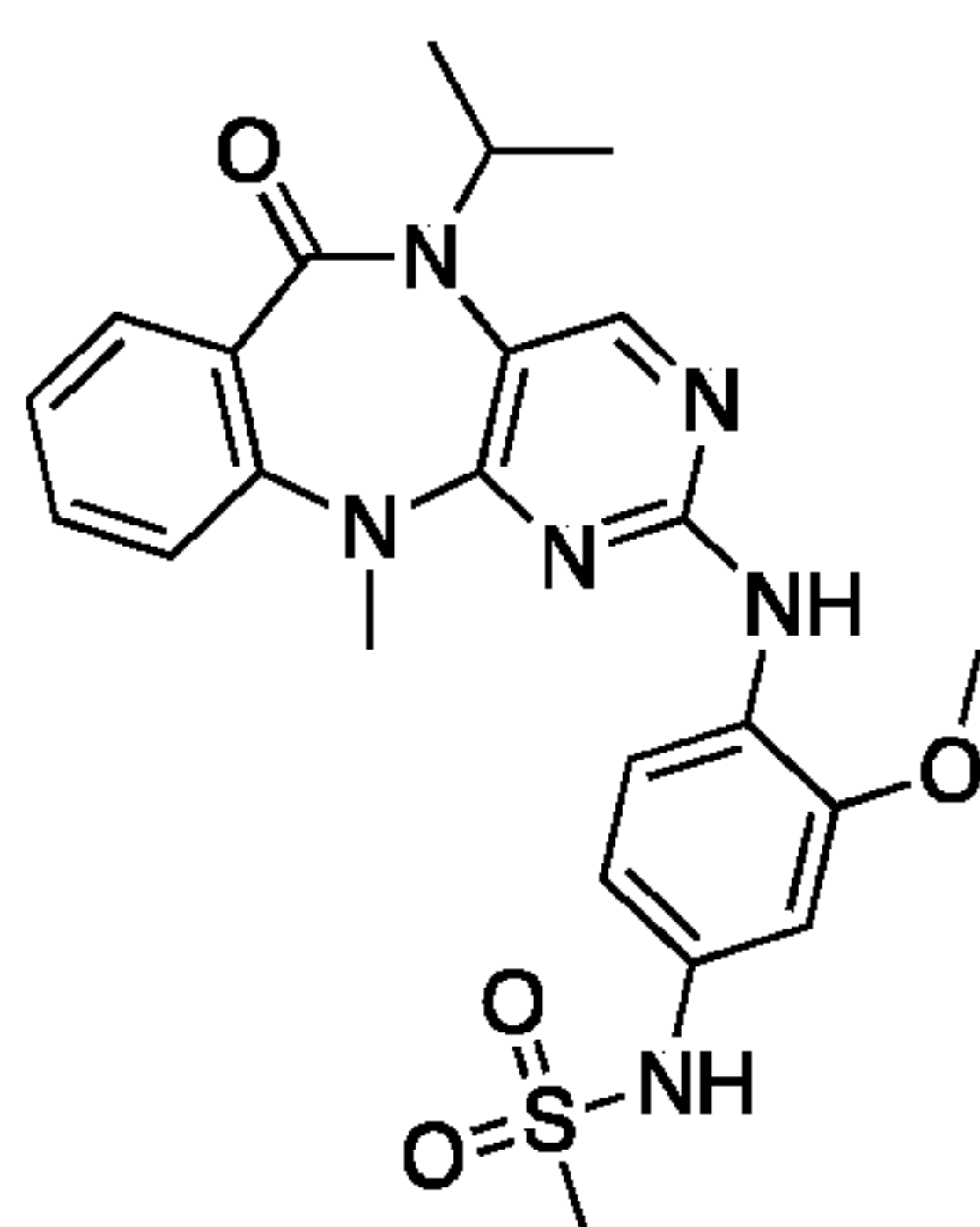
Compound 13: N -(4-((5-isopropyl-11-methyl-6-oxo-6,11-dihydro-5 H -benzo[ e ]pyrimido[5,4- b ][1,4]diazepin-2-yl)amino)-3-methoxyphenyl)methanesulfonamide (FMF-03-150-2)
