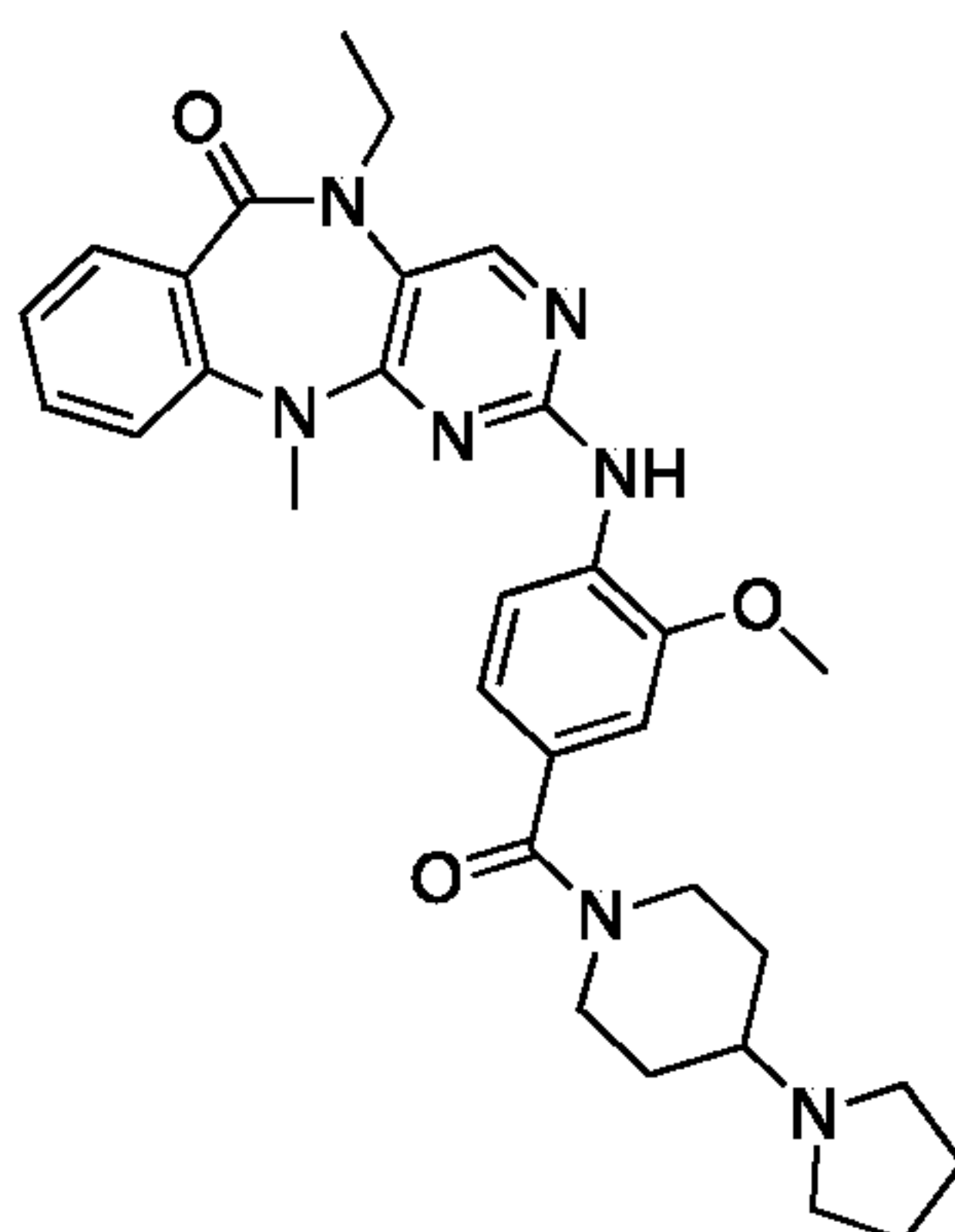
Compound 14: 5-ethyl-2-((2-methoxy-4-(4-(pyrrolidin-1-yl)piperidine-1-carbonyl)phenyl)amino)-11-methyl-5,11-dihydro-6 H -benzo[ e ]pyrimido[5,4- b ][1,4]diazepin-6-one (FMF-03-058-2)
