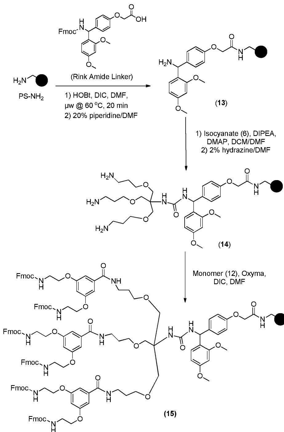
Scheme 3: Synthesis of 3 and 6-branched dendrimeric scaffolds (14) and (15)
