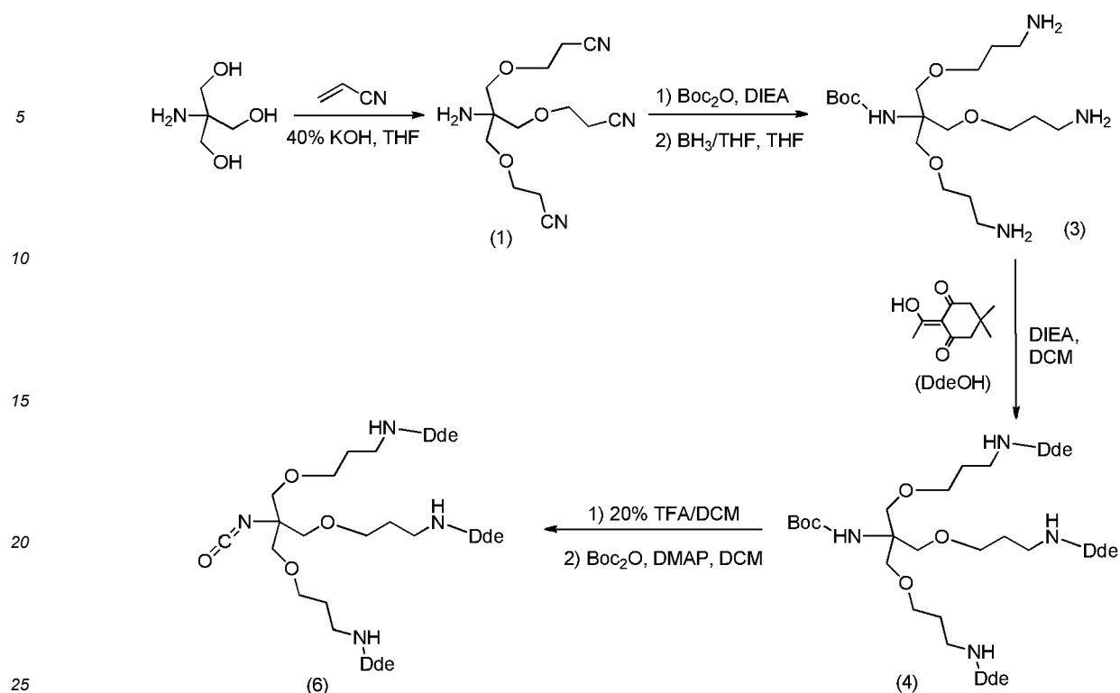
Scheme 1: Synthesis of monomer (6)
