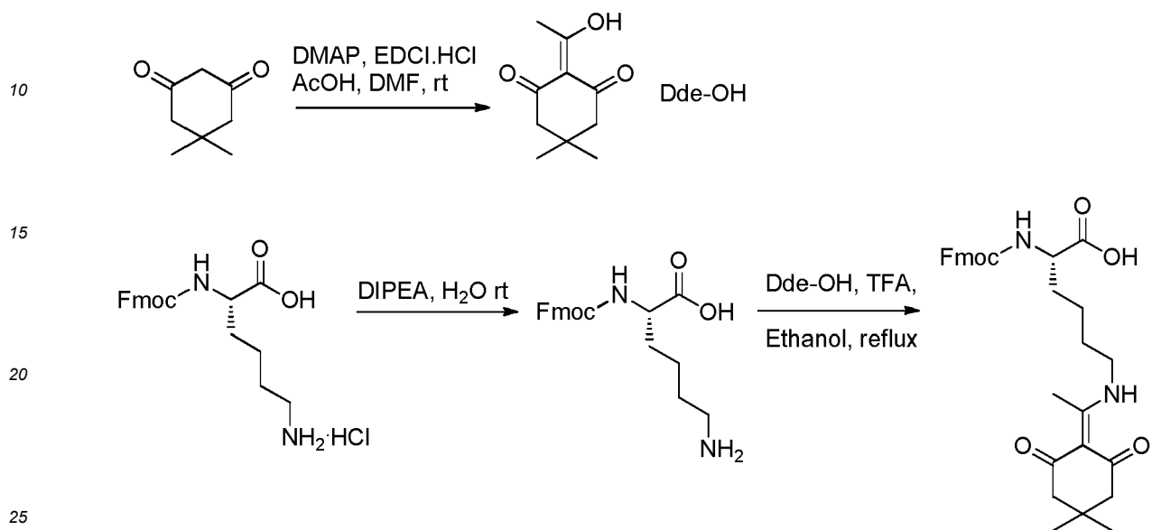
Scheme 1: Synthesis of Fmoc-Lys(Dde)-OH
