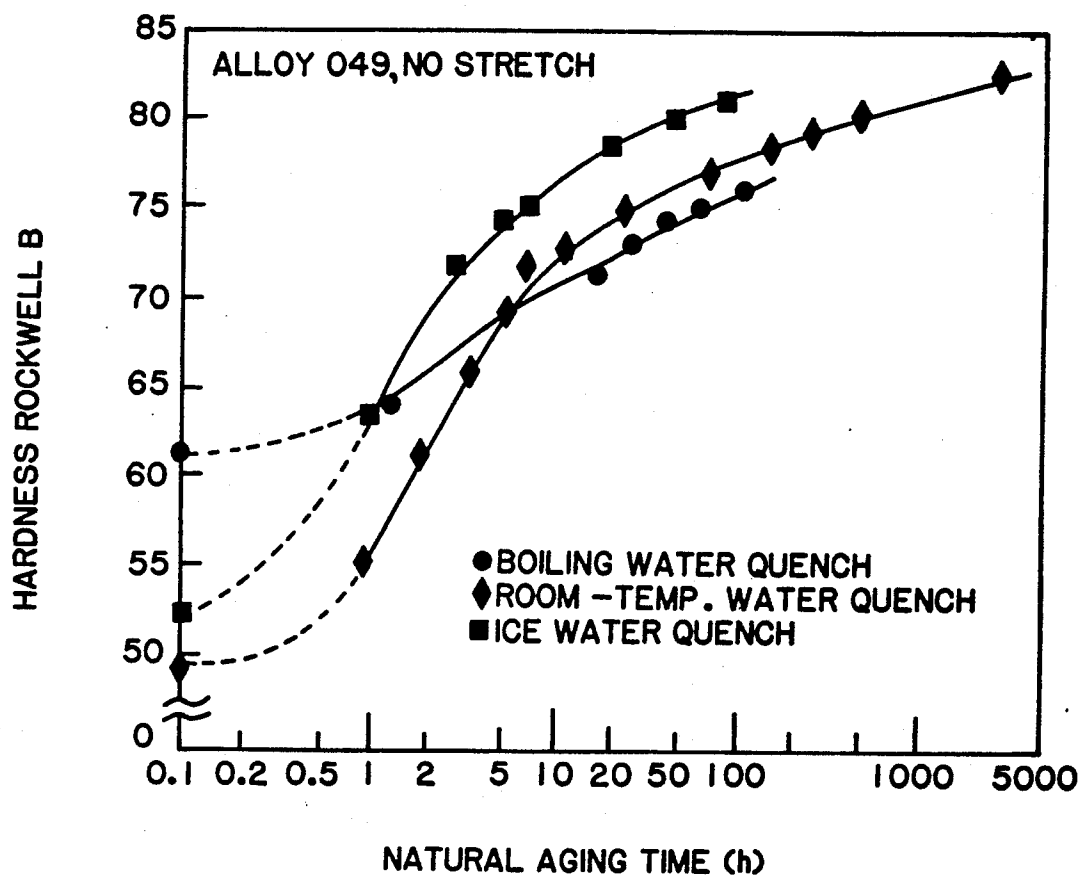
NATURAL AGING RESPONSE OF UNSTRETCHED 049 ALLOY AFTER QUENCHING FROM 504°C INTO VARIOUS MEDIA
