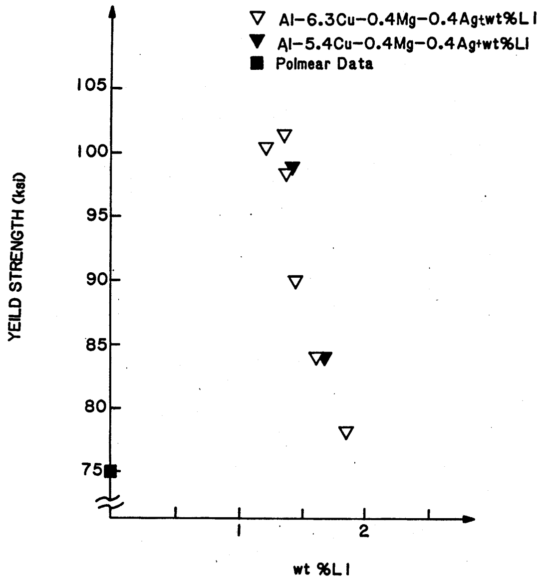
YIELD STRENGTH VS. WEIGHT PERCENT LITHIUM OF AL-CU BASED ALLOYS IN THE SUA TEMPER
