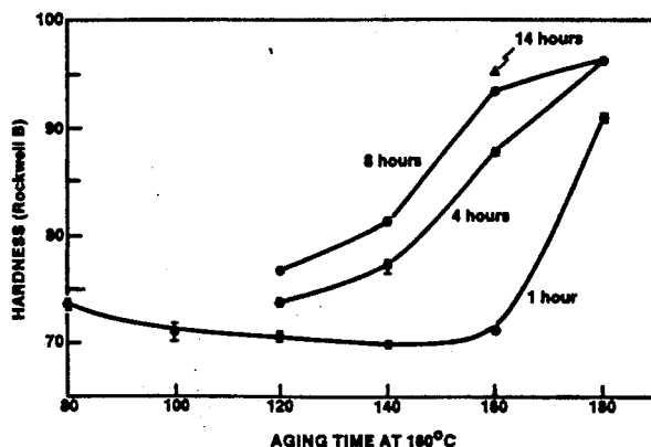
ISOCHRONAL AGING CURVES FOR AL-CU-MG-AG-LI ALLOY 019
