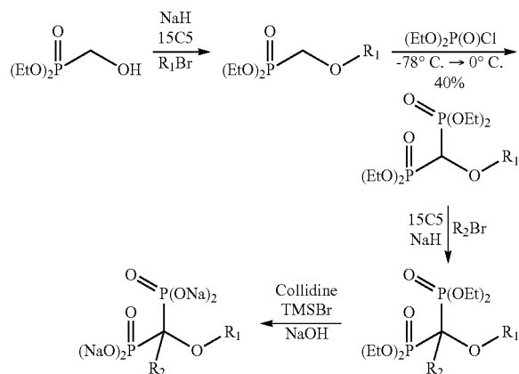
Scheme 1. General preparation of compounds.
