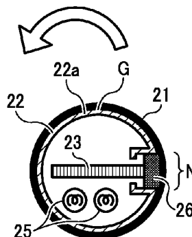
ROTATION DIRECTION OF FIXING BELT
