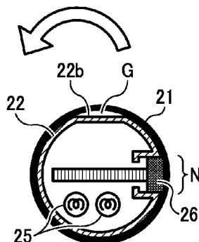
ROTATION DIRECTION OF FIXING BELT
