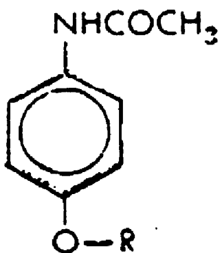
Conjugated Acetaminophen
