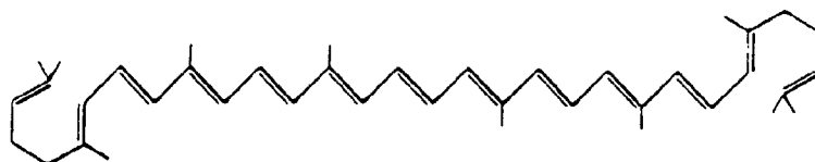
Lycopene
