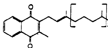
Phylloquinone
