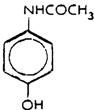
Acetaminophen
