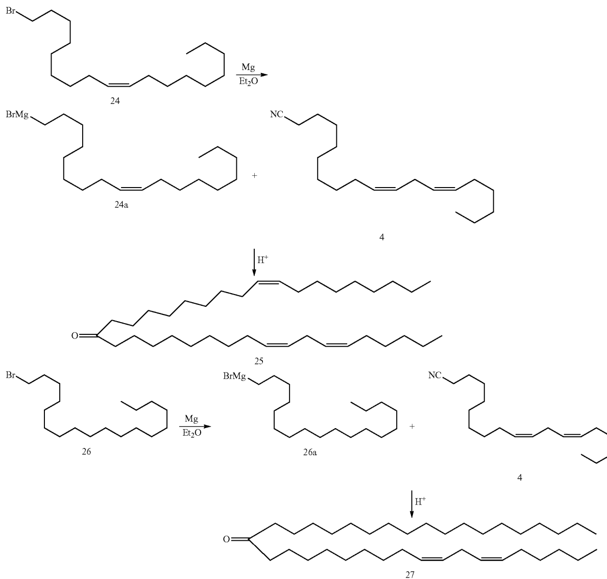
Scheme 3
