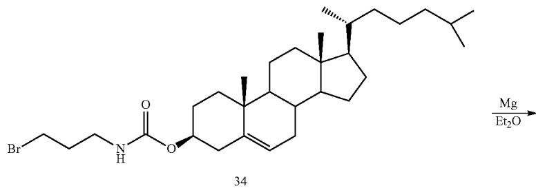
Scheme 7
