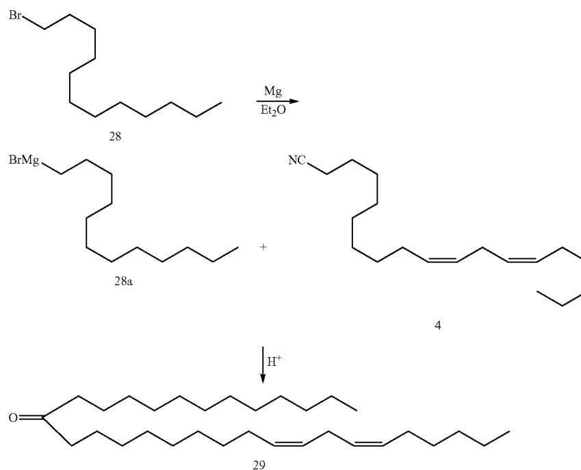
Scheme 4
