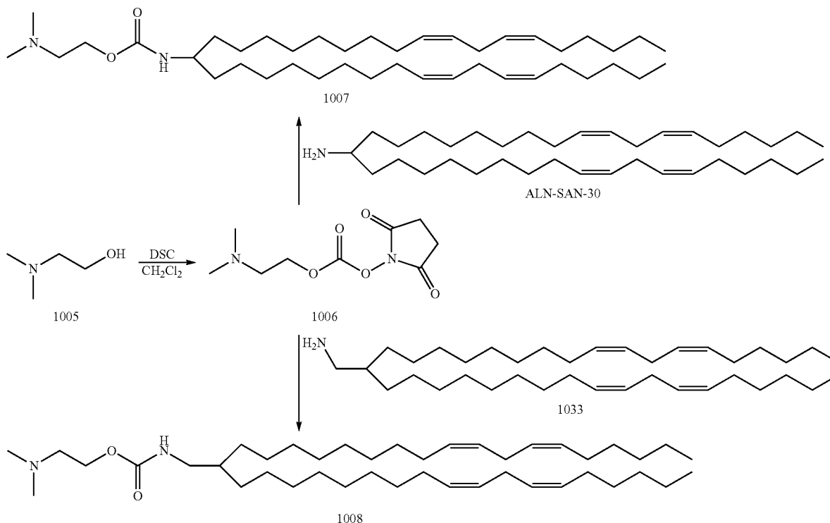
Scheme 3
