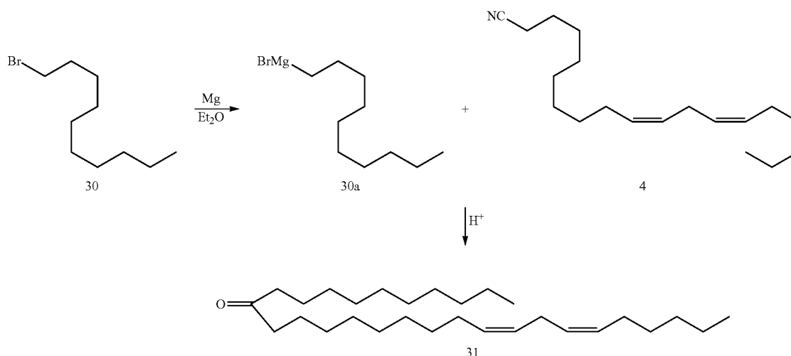
Scheme 5
