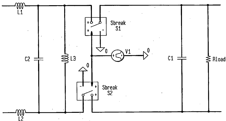
FIG. 242 DIFFERENTIAL CONFIGURATION
