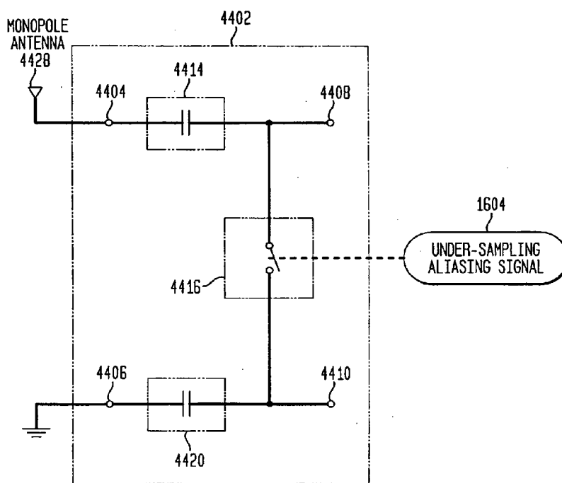
FIG. 44C SINGLE INPUT TO DIFFERENTIAL OUTPUT
