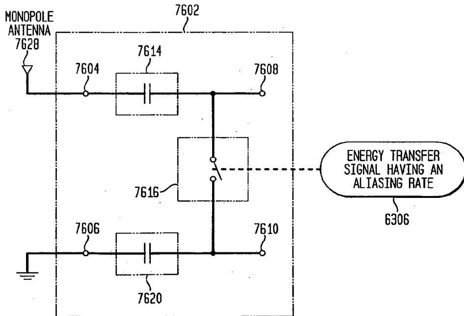
FIG. 76C SINGLE INPUT TO DIFFERENTIAL OUTPUT
