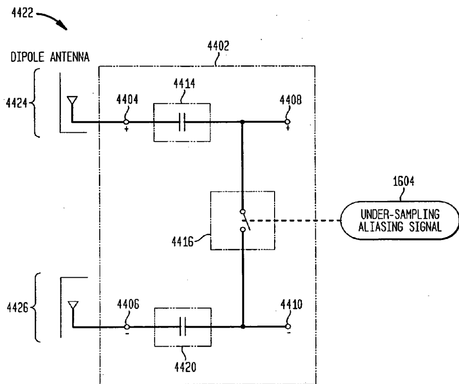
FIG. 44B DIFFERENTIAL INPUT TO DIFFERENTIAL OUTPUT
