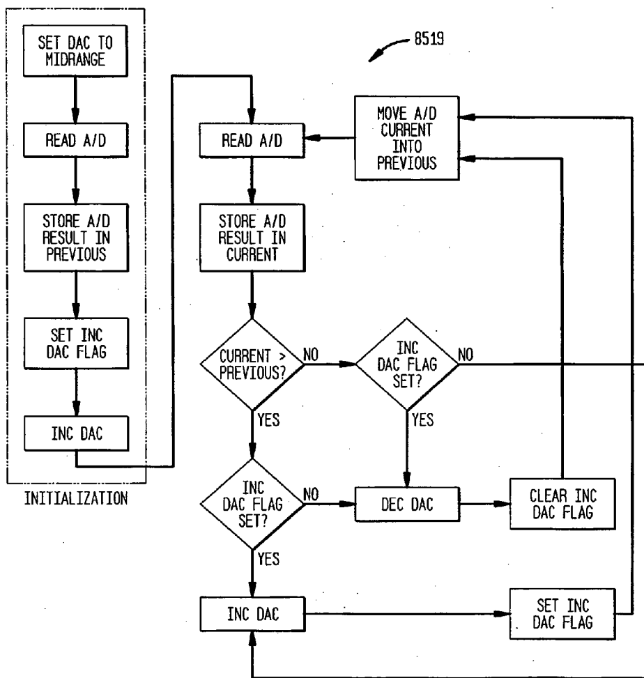
STATE MACHINE FLOWCHART
