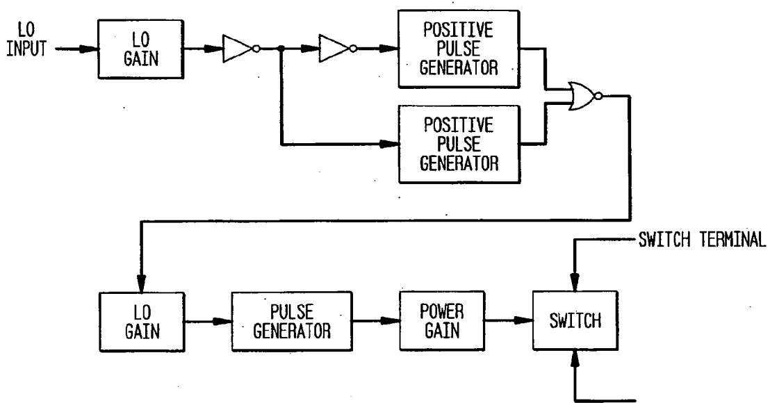
CMOS "HOT CLOCK" BLOCK DIAGRAM
