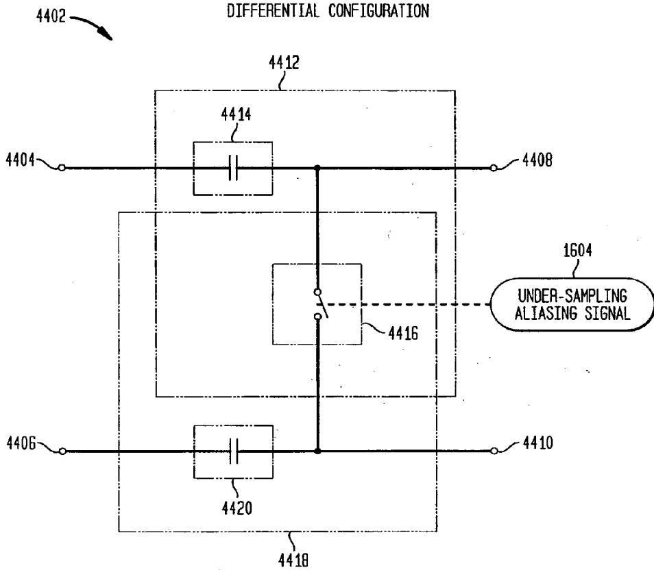
FIG. 44A DIFFERENTIAL CONFIGURATION
