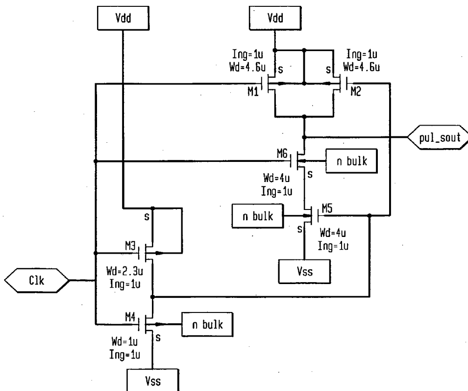
PULSE GENERATOR#1 AT TRANSISTOR LEVEL
