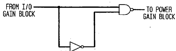
PULSE GENERATOR#1 AT GATE LEVEL
