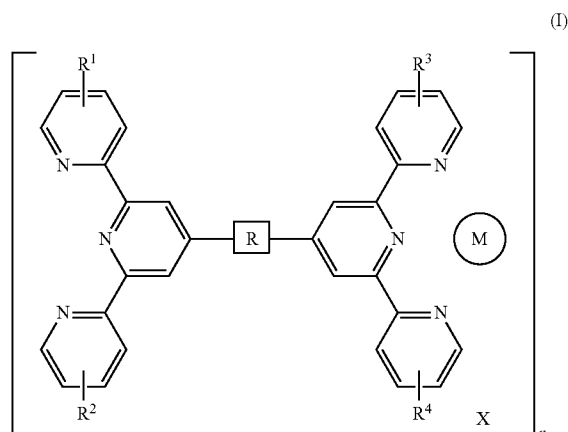
[Chemical Formula 3]
