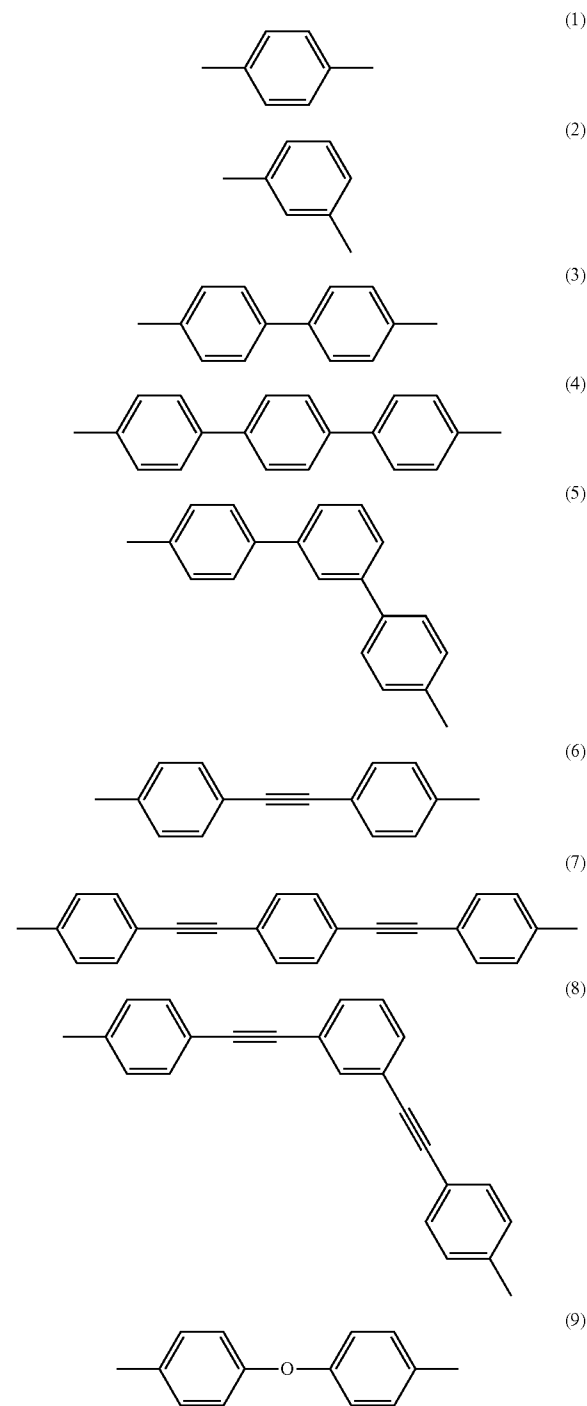
[Chemical Formula 5]
