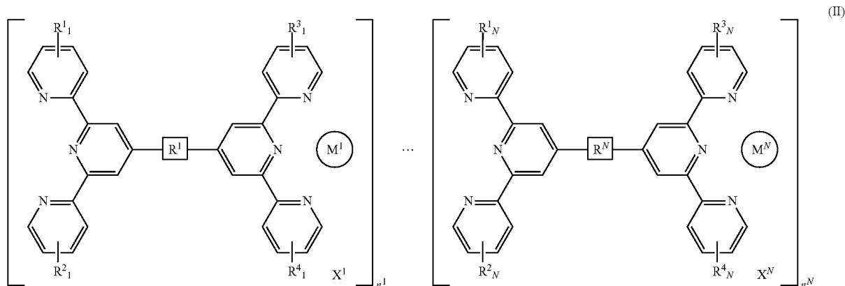
[Chemical Formula 2]
