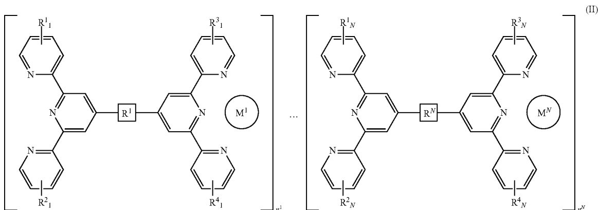
[Chemical Formula 4]
