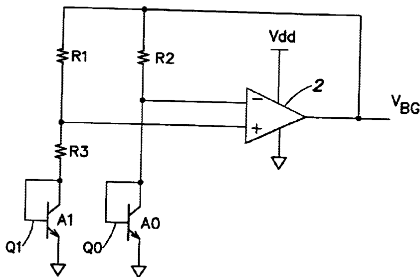
FIG. 2 (PRIOR ART)
