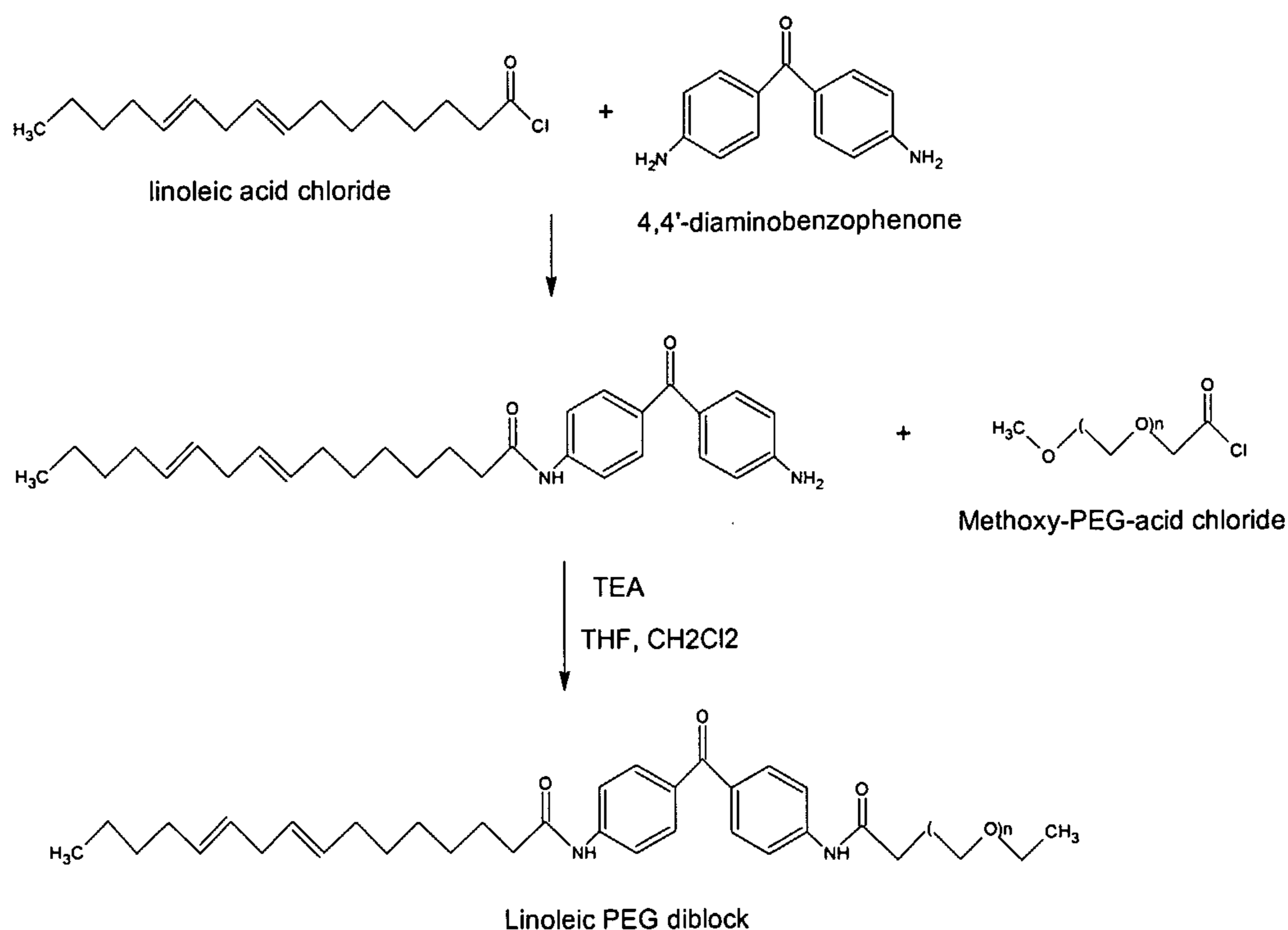
Figure 1. Synthesis of linoleamide PEG (where TEA = triethylamine)
