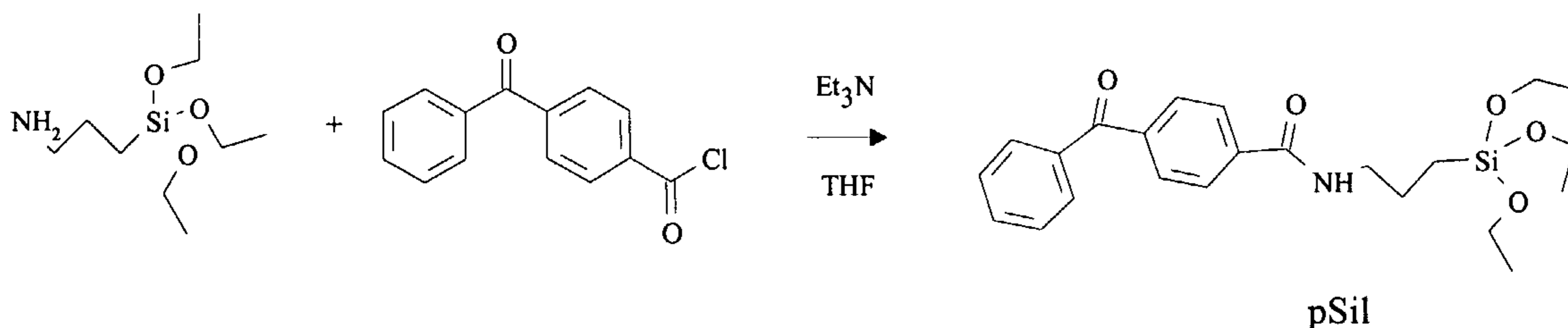
20 Figure 10. Synthesis of photosilane reagent, pSil.
