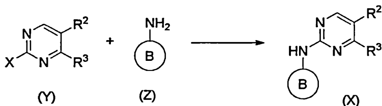
Scheme I
