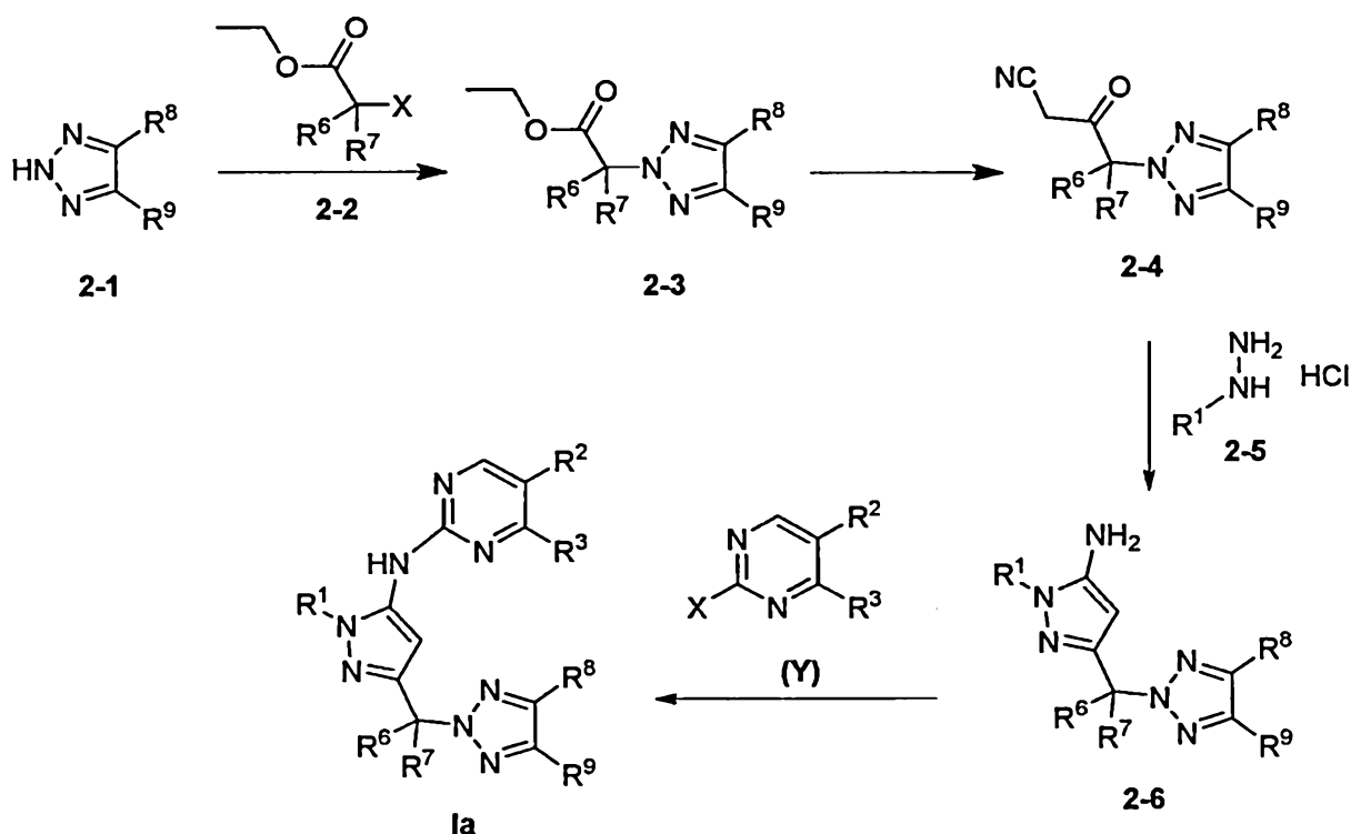
Scheme II
