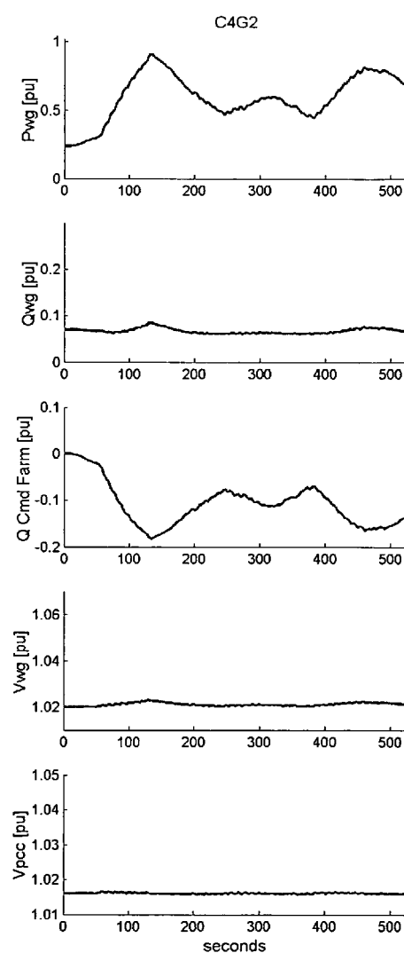
Fig. 5 PRIOR ART
