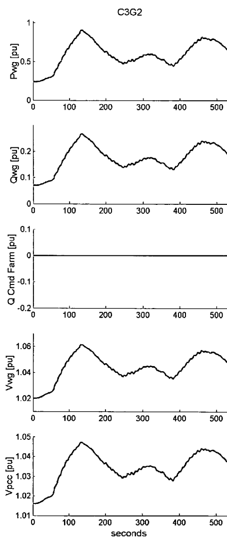
Fig. 4 PRIOR ART
