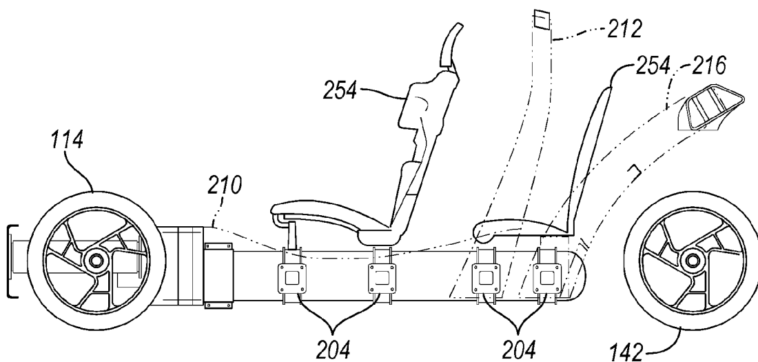
SIDE STRUCTURE
