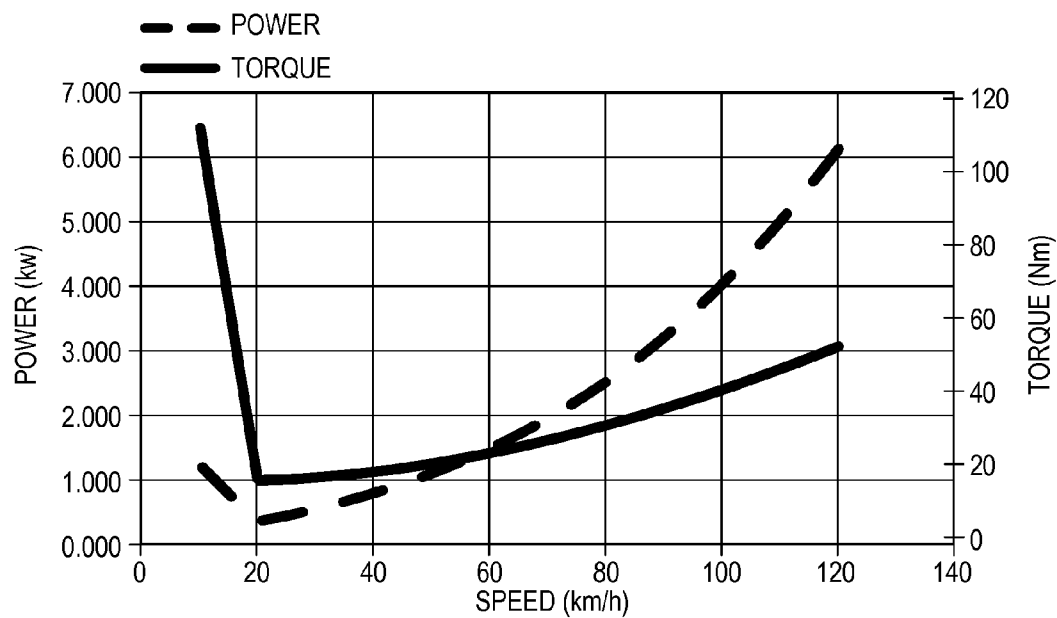
REQUIRED POWER AND TORQUE CURVES
