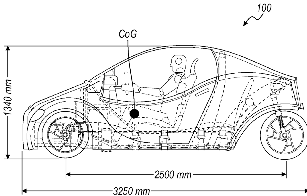
VEHICLE DIMENSIONS
