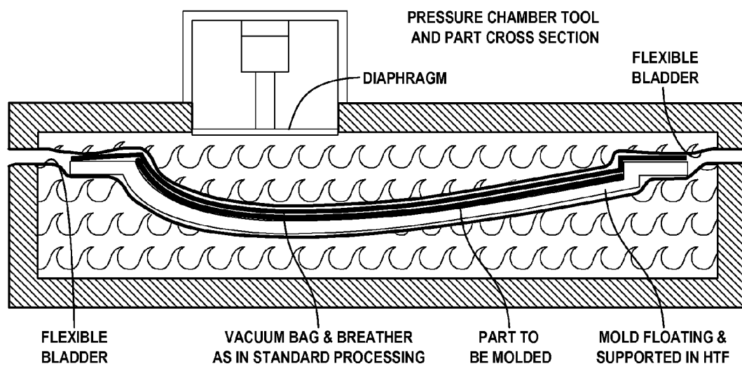
SCHEMATIC OF THE COMPOSITE LAYER PROCESS
