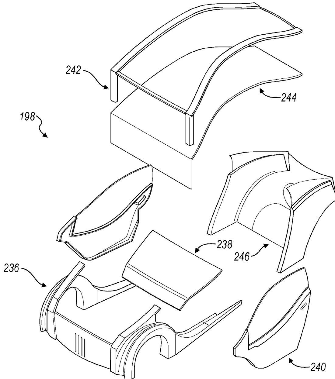
UPPER VEHICLE BODY EXPLODED VIEW
