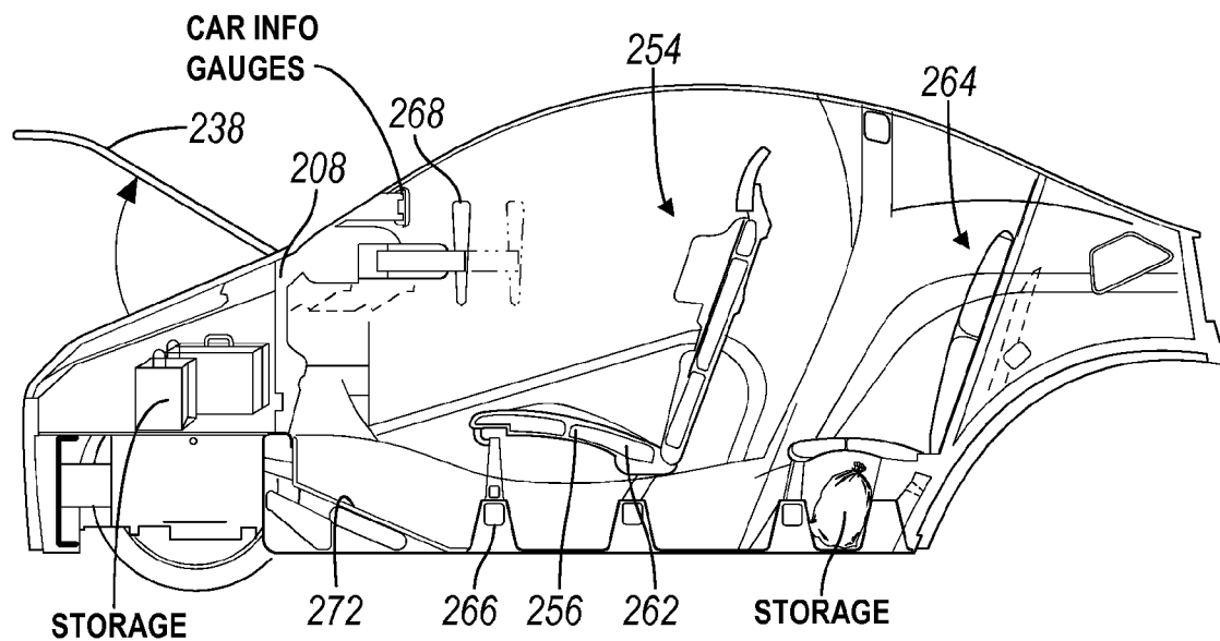
SECTIONAL VIEW OF VEHICLE INTERIOR.
