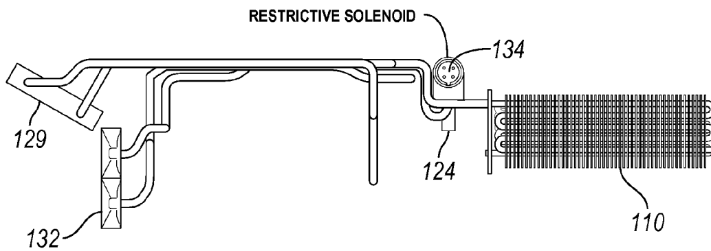
ANOTHER VIEW OF THE HVAC CONNECTIONS
