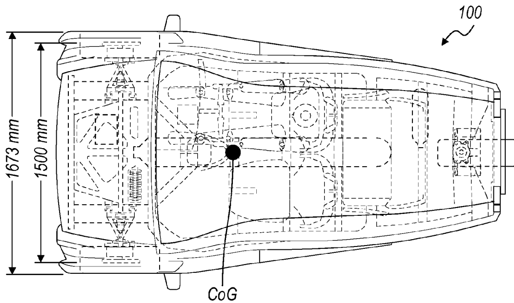
VEHICLE DIMENSIONS
