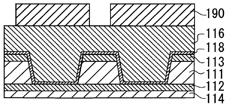
Fig.69 PRIOR ART
