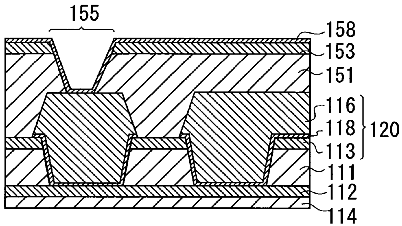
Fig. 73 PRIOR ART
