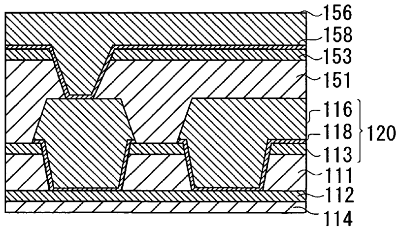
Fig. 74 PRIOR ART
