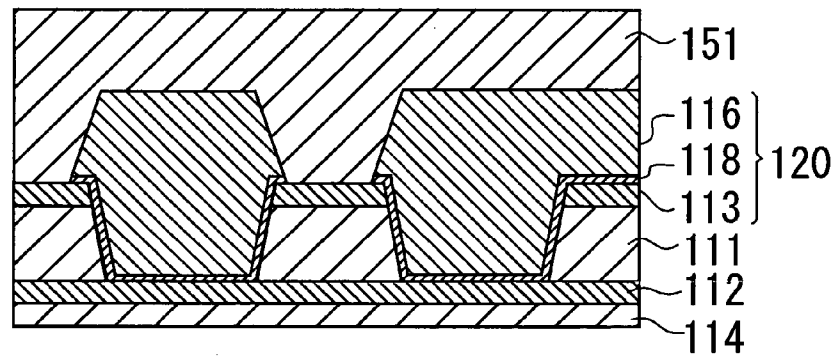
Fig.71 PRIOR ART
