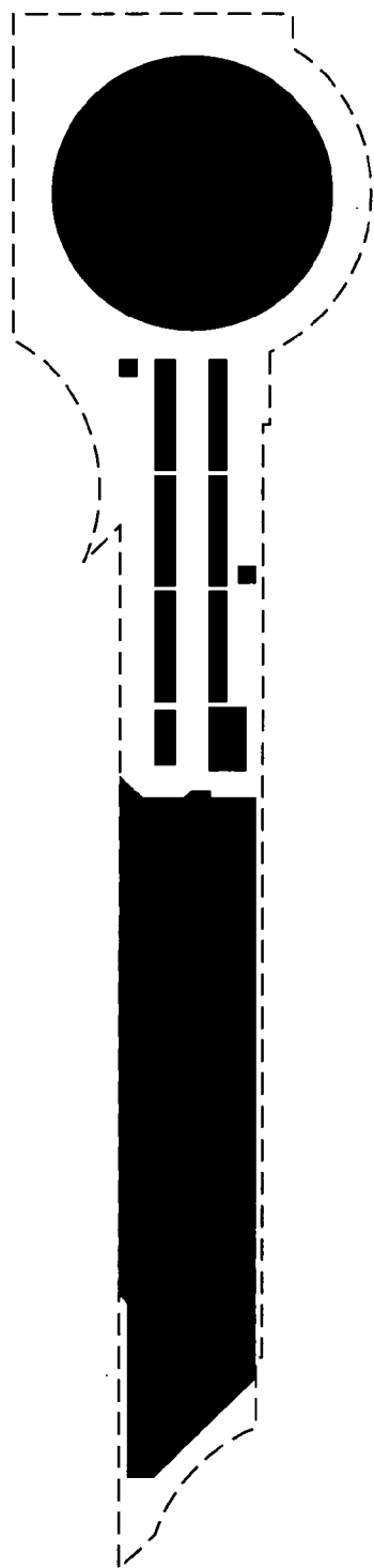
Active mask
