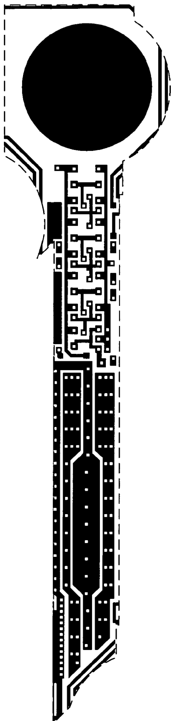
Metal 1 mask
