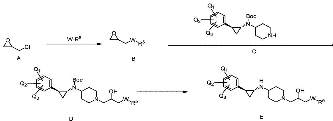
Scheme Ib
