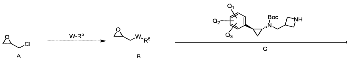
Scheme Ia
