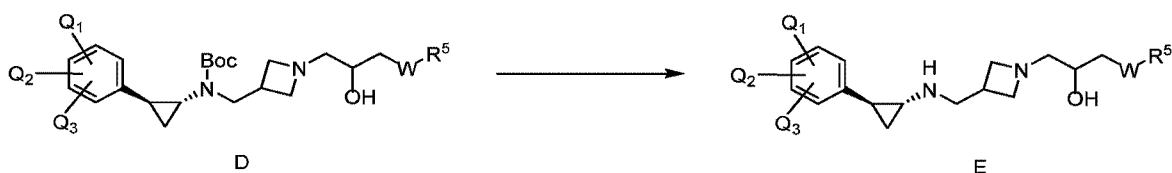
Scheme Ib
