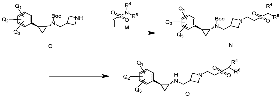
Scheme IVa
