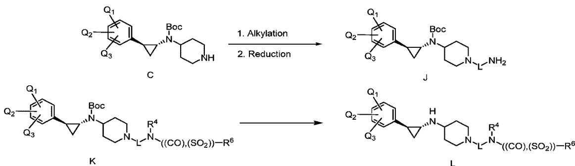
Scheme IIIb
