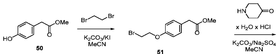
Scheme 15
