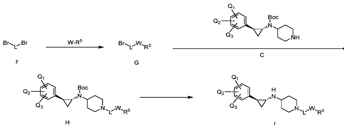
Scheme IIb
