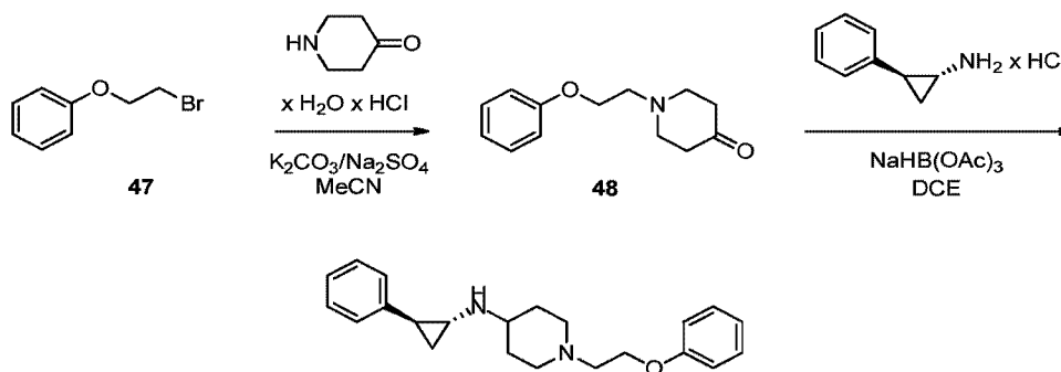
Scheme 14
