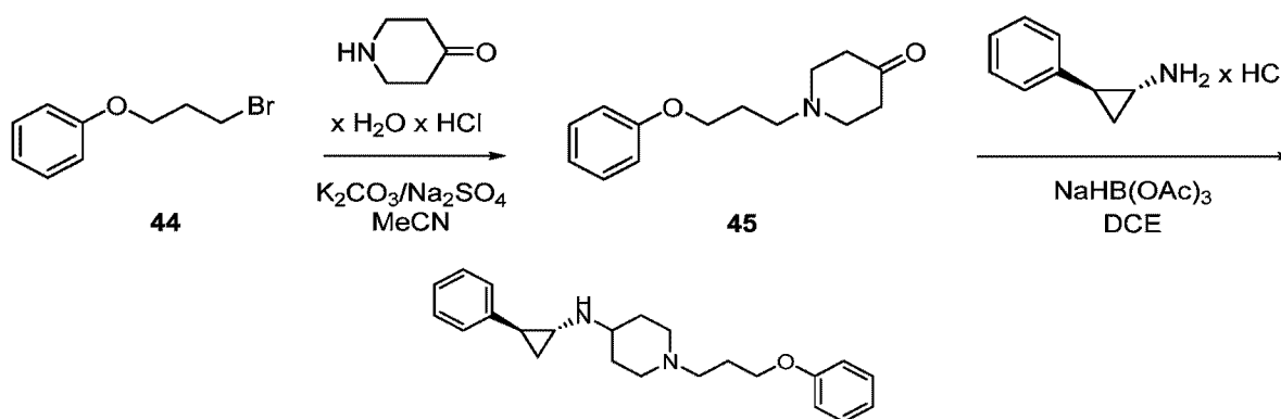
Scheme 13
