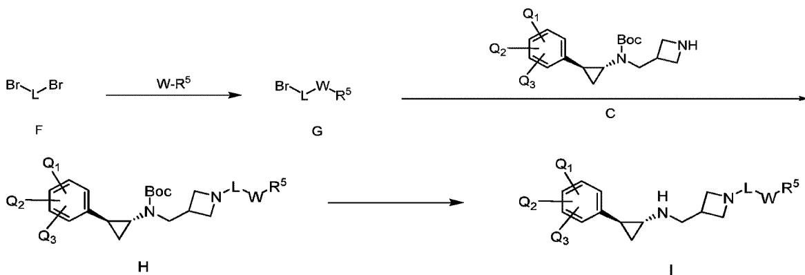
Scheme IIa
