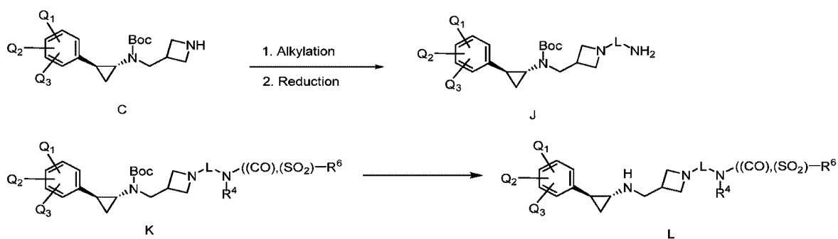
Scheme IIIa
