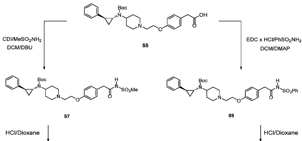
Scheme 16
