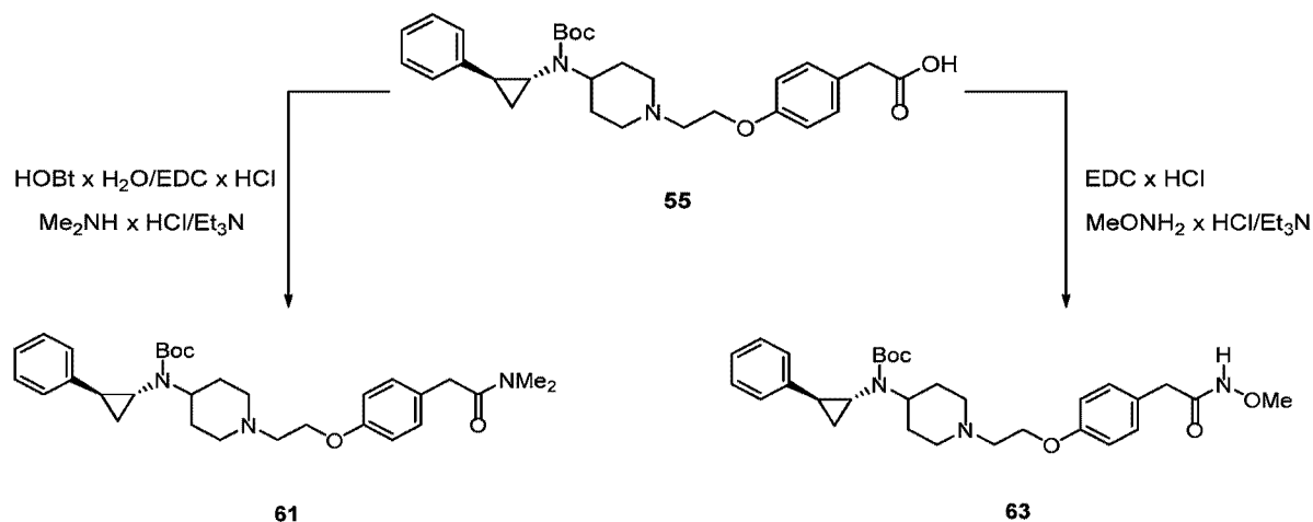
Scheme 17
