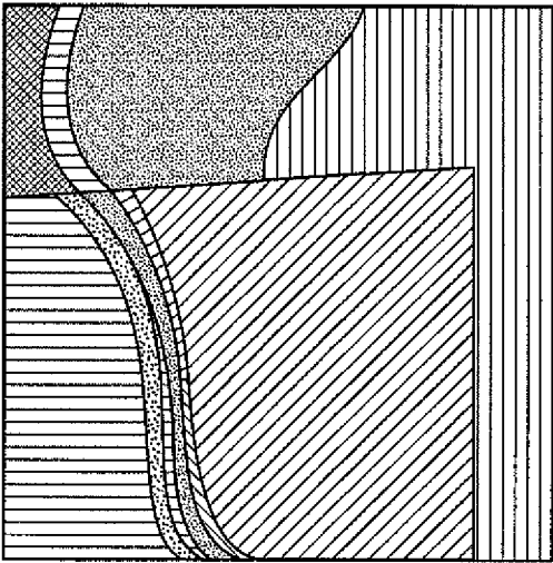
Token Regions
