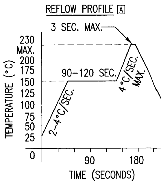
FIG. 1c PRIOR ART
