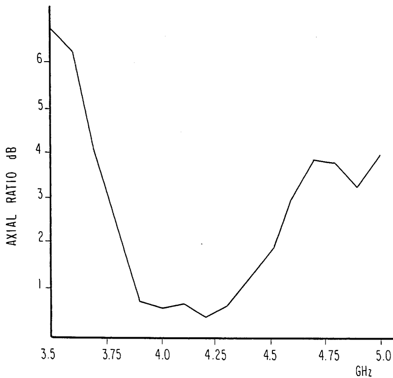
FIG. 7 - AXIAL RATIO OF 4-ELEMENT ARRAY
