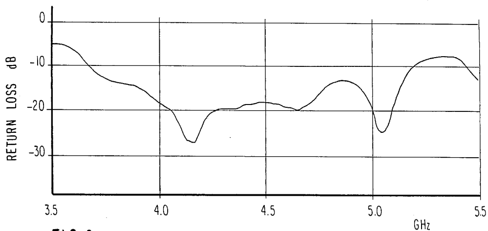
FIG. 6 - RETURN LOSS OF 4-ELEMENT CIRCULARLY POLARIZED CF-EMCP
