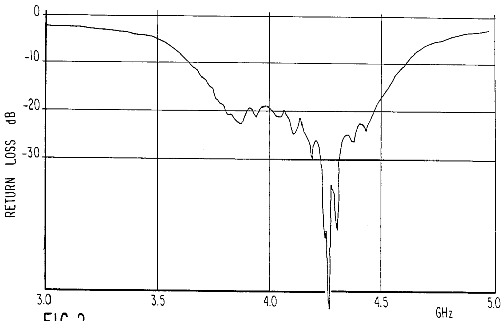
FIG. 2 - RETURN LOSS OF OPTIMIZED LINEARLY POLARIZED CF-EMCP ELEMENT
