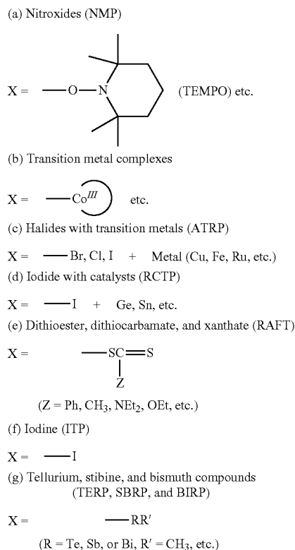
Scheme 2. Examples of capping agent X.
