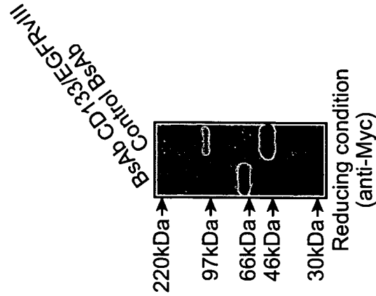
Western blot of purified BsAb
