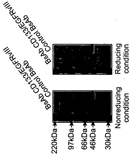
Coomassie staining of purified BsAb
